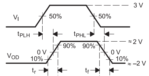
FIG 17. Measurement of Driver Differential Output Rise and Fall Times and Propagation Delays
