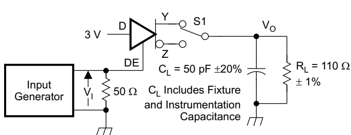
FIG 17. Measurement of Driver Differential Output Rise and Fall Times and Propagation Delays
