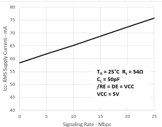
FIG 7-1. HVD50, HVD53 RMS Supply Current vs Signaling Rate
