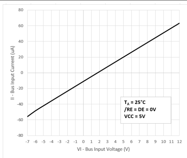
Figure 7-5. HVD51, HVD52, HVD54, HVD55 BUS Input Current vs Input Voltage
