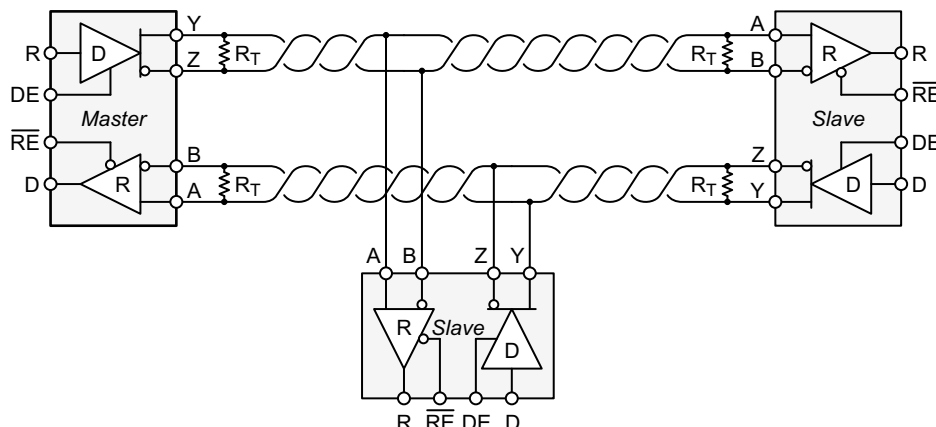
10-2. Typical RS-485 Network With Full-duplex Transceivers
