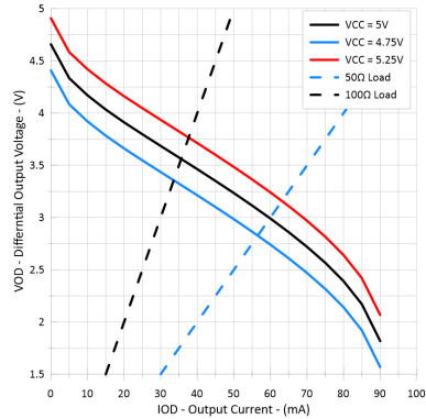
FIG 6-1. Differential Output Voltage vs Load Current
