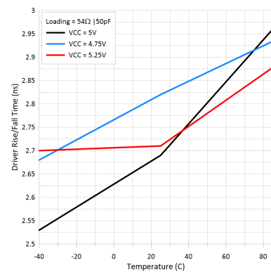
FIG 6-4. Driver Rise, Fall Time vs Free-Air Temperature
