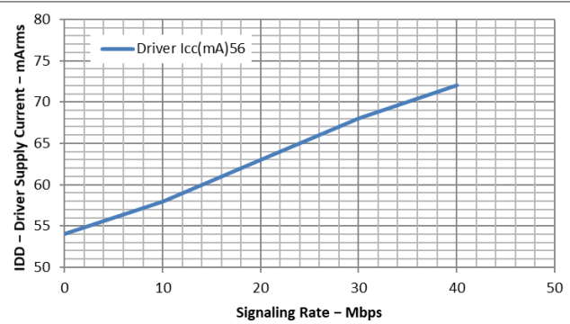
FIG 6-2. Driver Supply Current vs Signaling Rate
