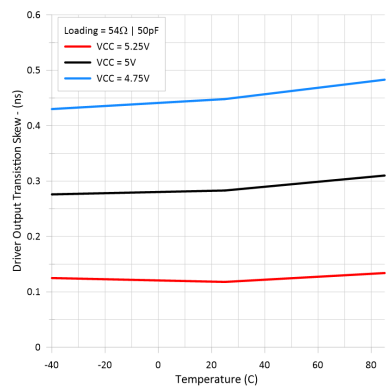
FIG 6-3. Driver Output Transition Skew vs Free-Air Temperature
