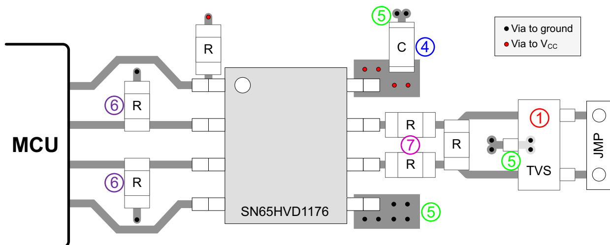
FIG 10-1. SNx5HVD08 Layout Example
