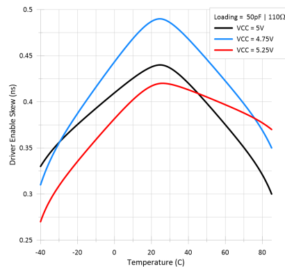
FIG 6-5. Driver Enable Skew vs Free-Air Temperature
