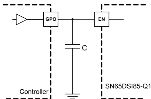
Figure 8. EN Input from Active Controller
