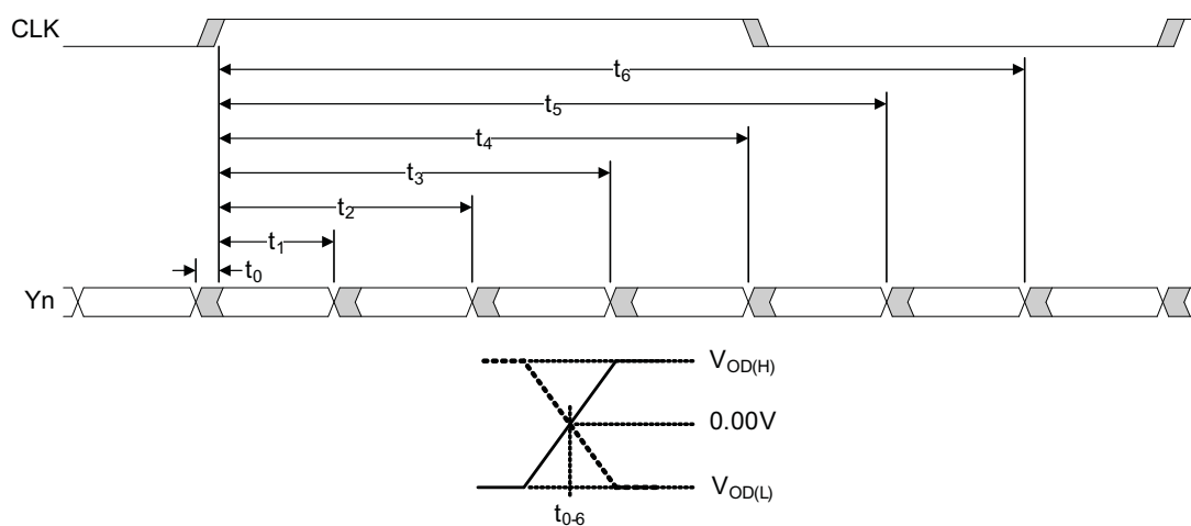
Figure 3. SN65DSI84-Q1 LVDS Timing Definitions
