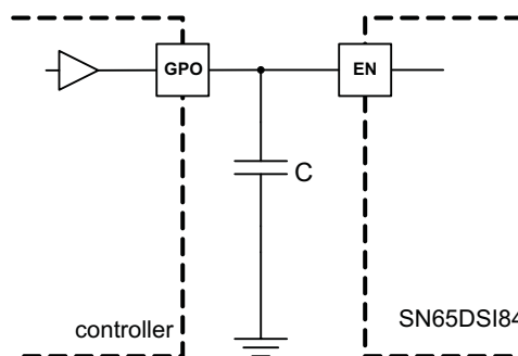
Figure 7. EN Input From Active Controller
