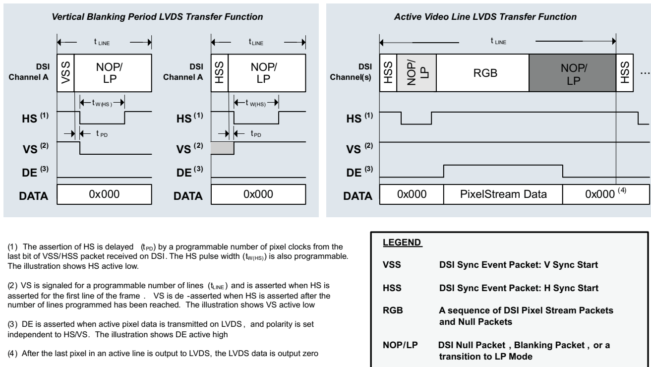
Figure 16. DSI Channel Transmission and Transfer Function
