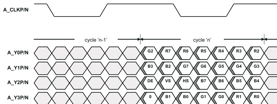
図 7-5. FlatLink Output Data (Format 2); Single-Link 24 bpp
