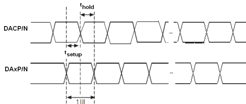
Fig 6-1. DSI HS Mode Receiver Timing Definitions
