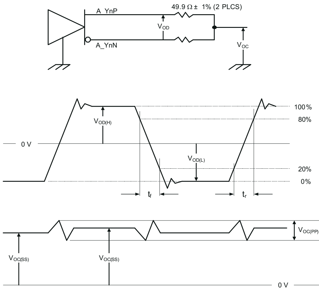
6-3. Test Load and Voltage Definitions for FlatLink Outputs
