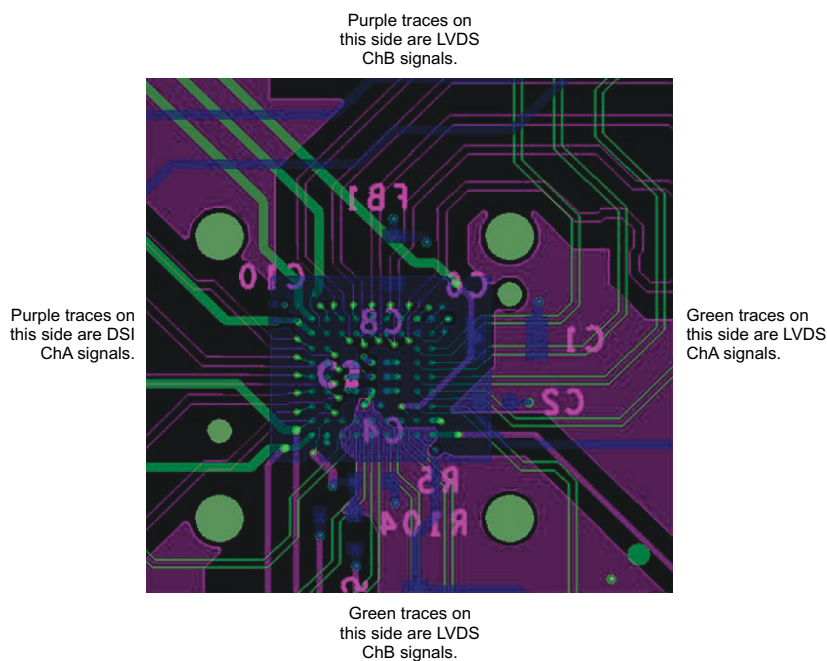
10-1. SN65DSI8x Layout Example
