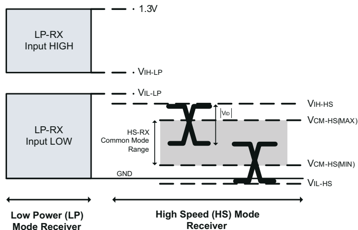
6-2. DSI Receiver Voltage Definitions
