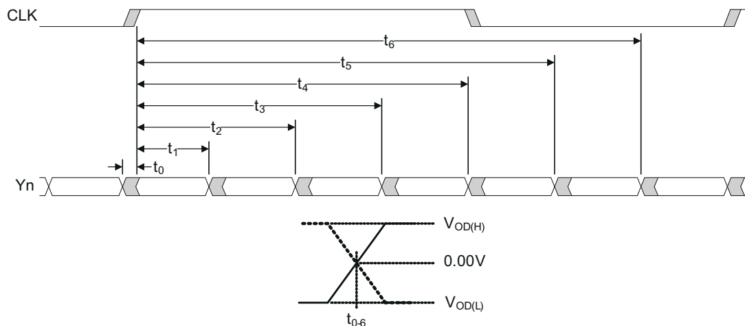
6-4. SN65DSI83 FlatLink Timing Definitions
