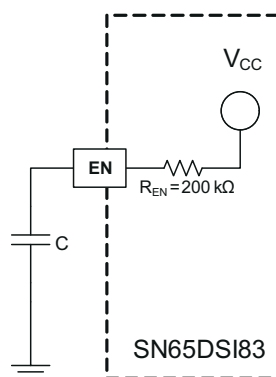
図 7-2. External Capacitor Controlled EN
