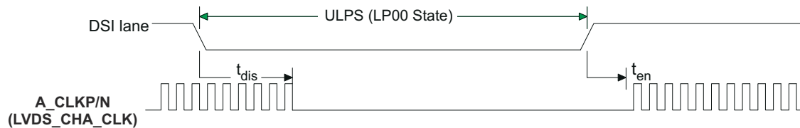
6-4. SN65DSI83 FlatLink Timing Definitions
