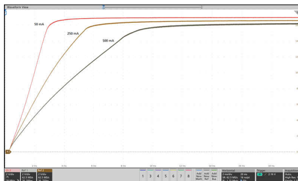
6-14. Output Voltage During Soft Start with 50-mA, 250-mA, and 500-mA Loads
