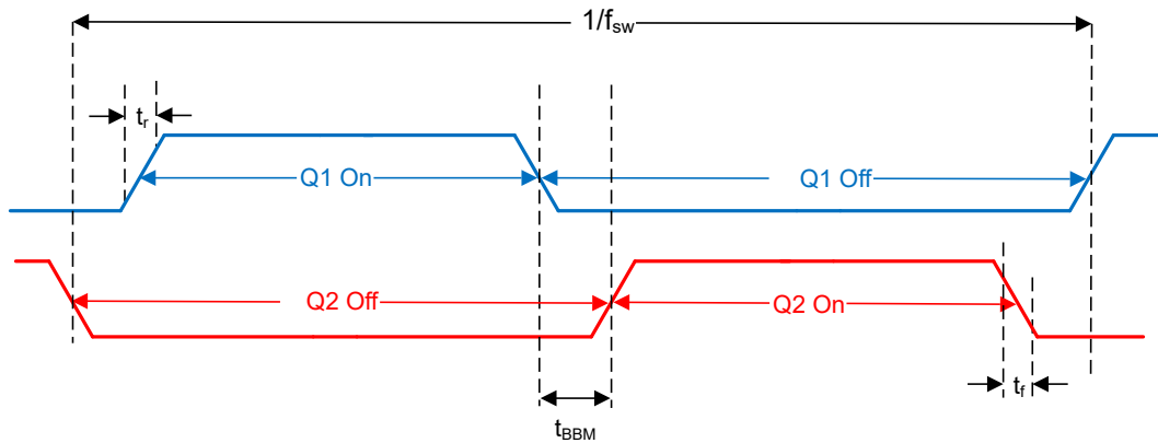
FIG 7-2. Timing Diagram
