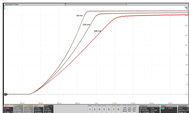
6-13. Output Voltage During Soft Start with 50-mA, 250-mA, and 500-mA Loads
