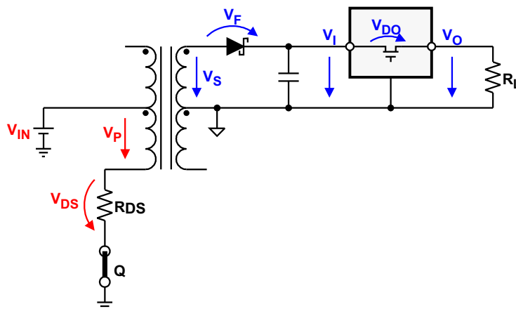
9-5. Establishing the Required Minimum Turns Ratio Through N_{\min} = 1.03 \times V_{S-\min} / V_{P-\min}
