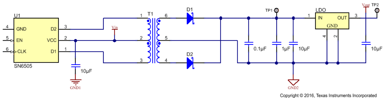
図 9-8. Regulated Output for Stable Supplies and High Current Loads
