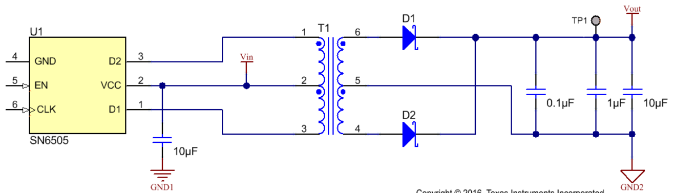
図 9-7. Unregulated Output for Low-Current Loads With Wide Supply Range
