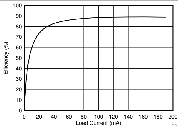
SN6505B + Würth 760390014 V_{CC} = 5\text{ V} D019
