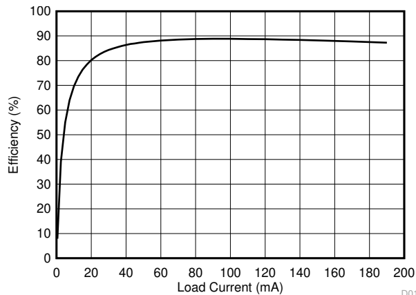
SN6505B + Würth 760390013 V_{CC} = 3.3\text{ V} D013
