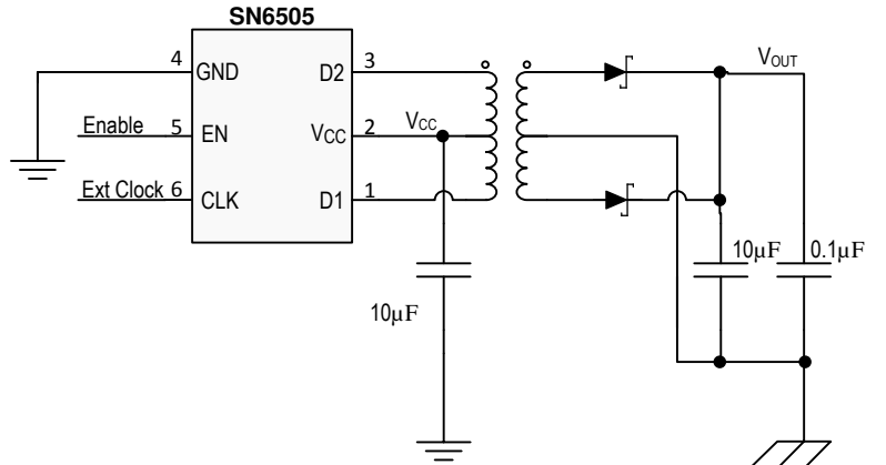
图 7-1. Measurement Circuit for Unregulated Output (TP1)
