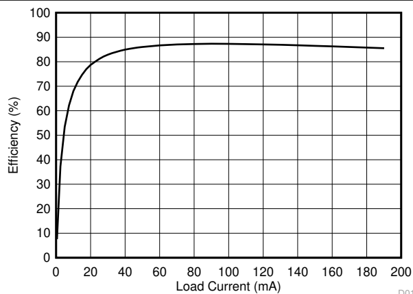
SN6505B + Würth 760390014 V_{CC} = 3.3\text{ V} D017
