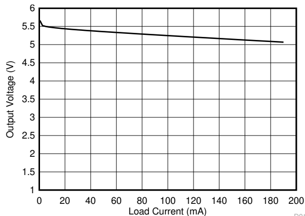
SN6505B + Würth 760390013 V_{CC} = 3.3\text{ V} D014
