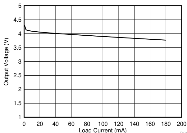
SN6505B + Würth 760390014 V_{CC} = 3.3\text{ V} D016
