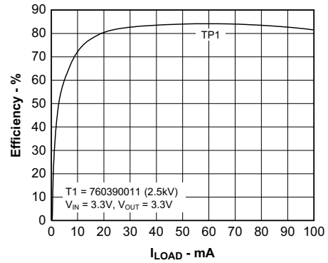
図 5-2. Efficiency vs Load Current
