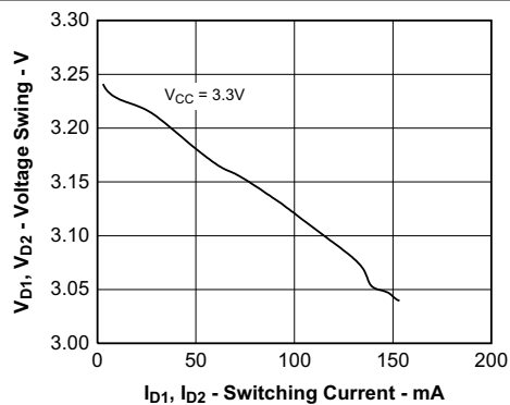
FIG 5-31. D1, D2 Primary-Side Output Switch Voltage Swing vs Current
