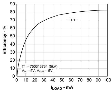
5-18. Efficiency vs Load Current
