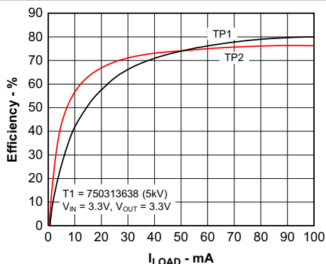
5-22. Efficiency vs Load Current
