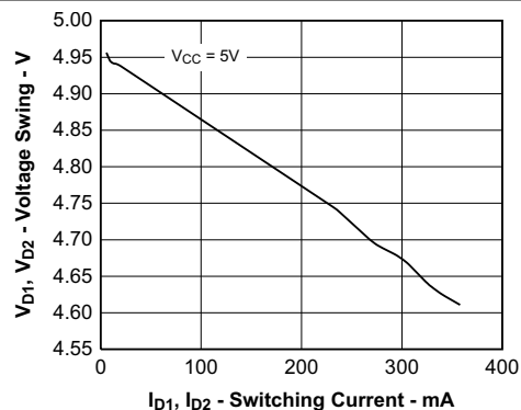
FIG 5-32. D1, D2 Primary-Side Output Switch Voltage Swing vs Current
