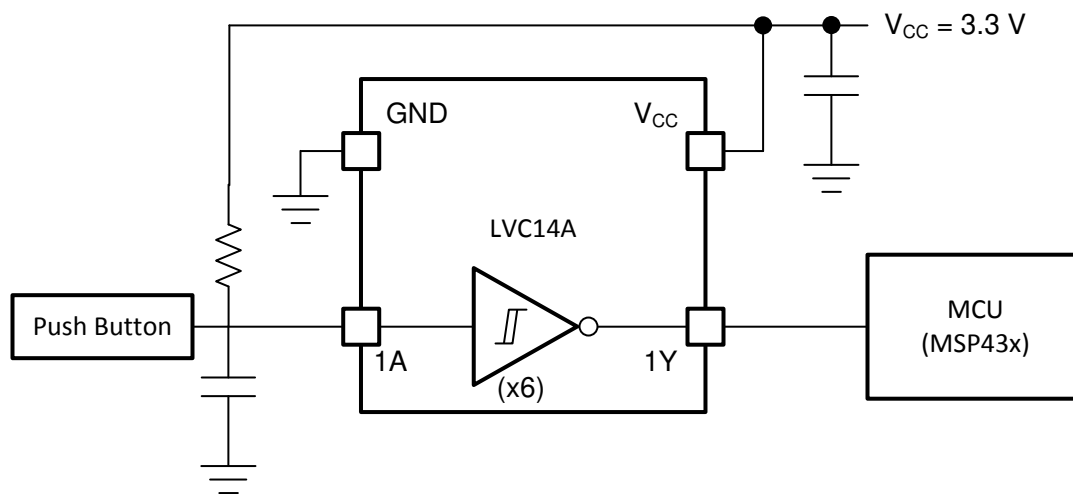
図 9-1. Debouncer Application Diagram
