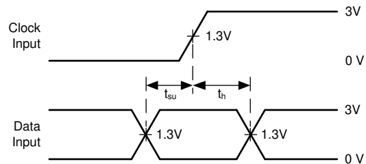
FIG 6-3. Voltage Waveforms, TTL-Compatible CMOS Inputs Setup and Hold Times
