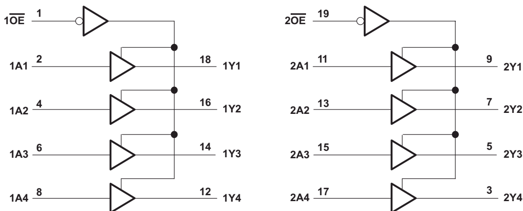
図 7-1. Logic Diagram (Positive Logic)
