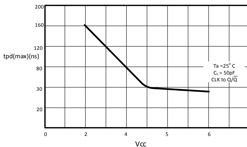
FIG 6-1. Max t_{pd} vs V_{CC}
