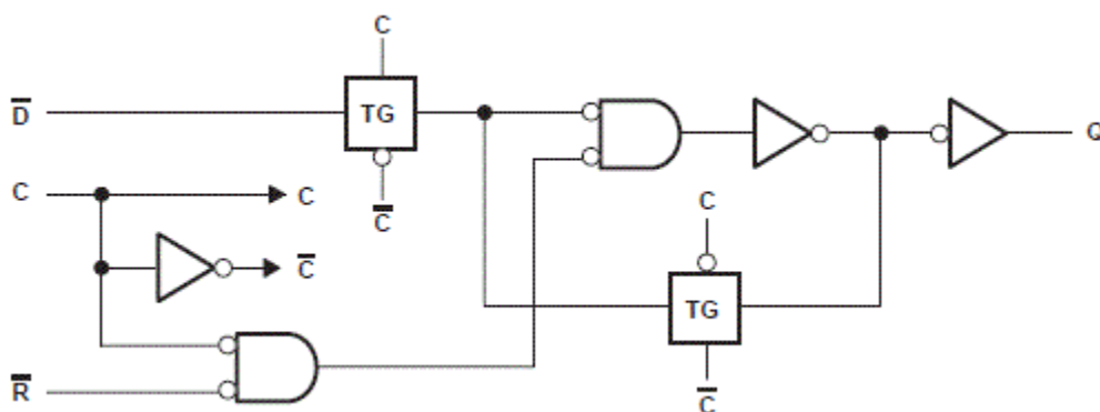
7-1. Logic Diagram, Each Internal Latch (positive logic)
