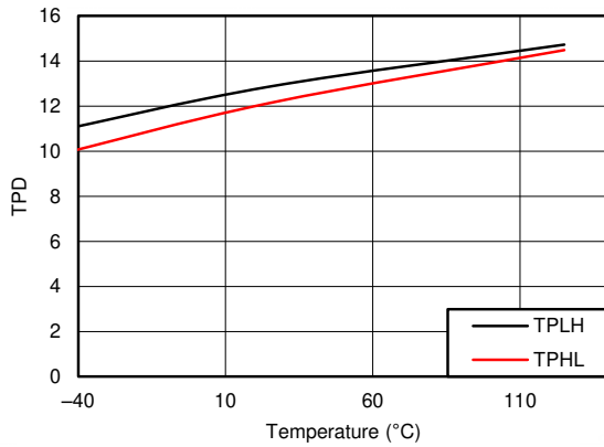
FIG 6-3. Typical propagation delay over temperature ( V_{CC} = 5\text{ V} )
