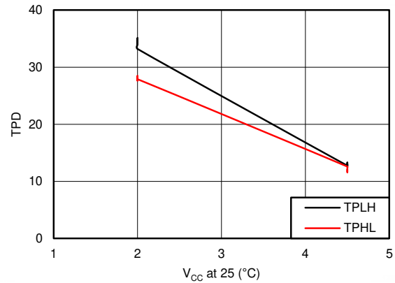
FIG 6-4. Typical propagation delay over supply ( V_{CC} at 25^\circ\text{C} )
