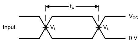
FIG 6-2. Voltage Waveforms, Pulse Duration
