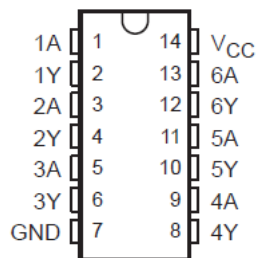
図 4-1. SN54ACT04 J or W Package; SN74ACT04 D, DB, N, NS, or PW Package Top View
