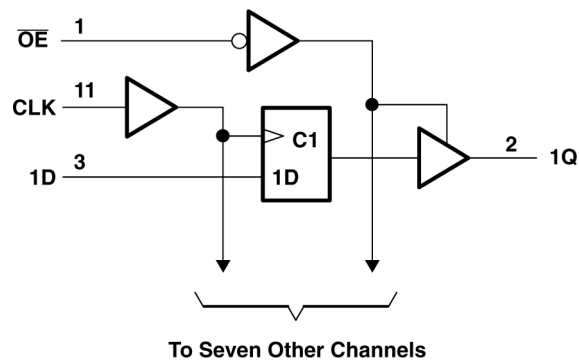
図 6-1. Logic Diagram (Positive Logic)
