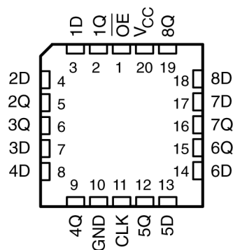
図 3-2. SN54AC374 FK Package (Top View)
