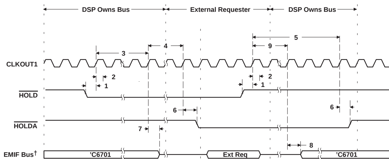
Figure 24. \overline{HOLD}/\overline{HOLDA} Timing
