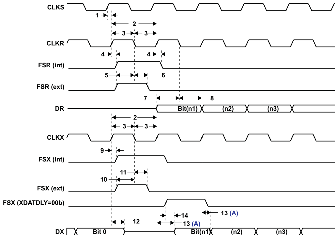
Figure 4-35. McBSP Timing
