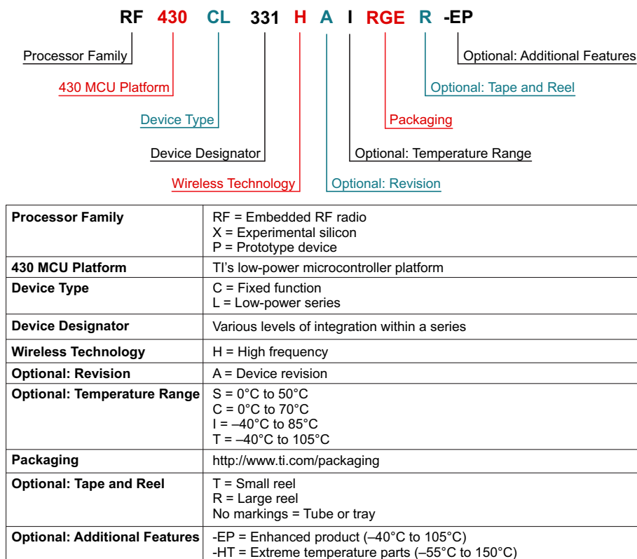
Figure 7-1. Device Nomenclature
