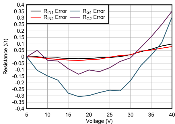
Figure 7-3. Resistor Actual-to-expected Mismatch vs Voltage
