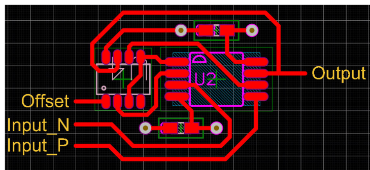
8-14. Single-Layer Instrumentation Amplifier Implementation
