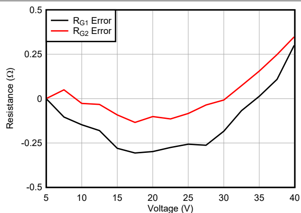
RES11A40-Q1 R_{Gx} actual – R_{Gx} predicted, normalized to R_{X(5V)}
