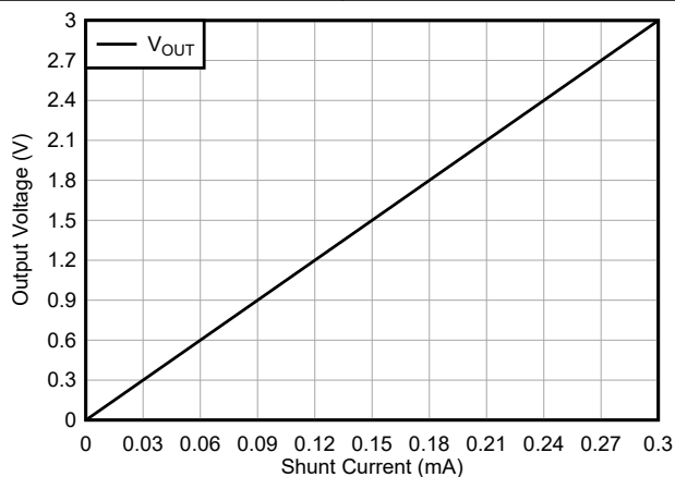
図 8-11. Simulation Result for V_{\text{OUT}}
