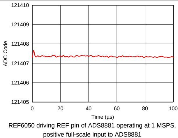
Figure 59. Reference Droop
