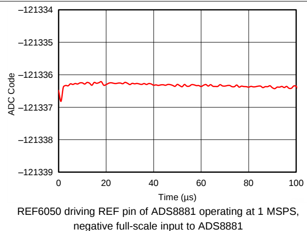
Figure 60. Reference Droop
