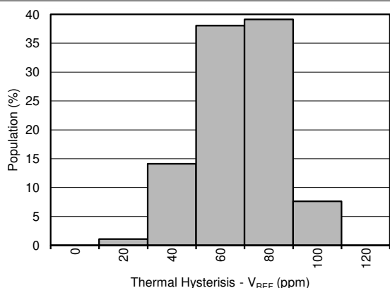
図 8-5. Thermal Hysteresis Distribution ( V_{\text{REF}} )
