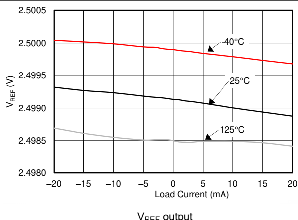
FIG 7-12. Output Voltage Change vs Load Current ( V_{REF} )
