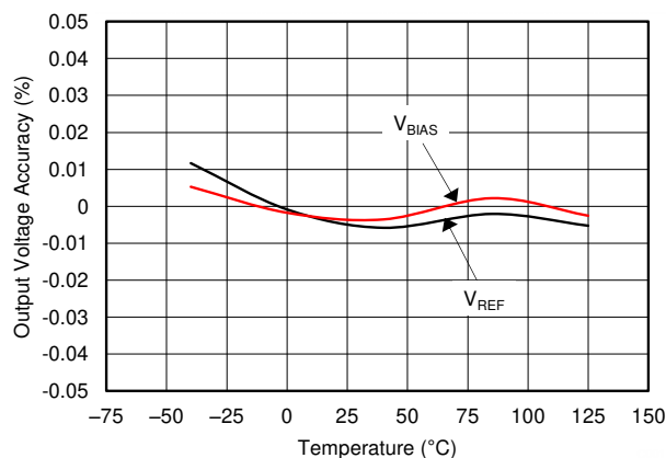
Figure 9-1. V_{REF} and V_{BIAS} Tracking vs Temperature
