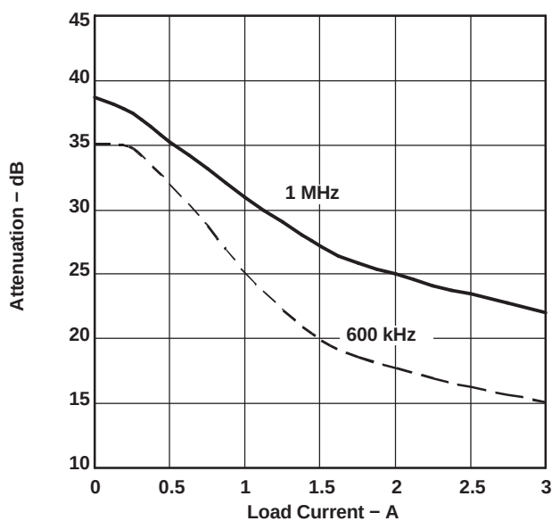
Figure 33. \pi -Filter Attenuation vs. Load Current
