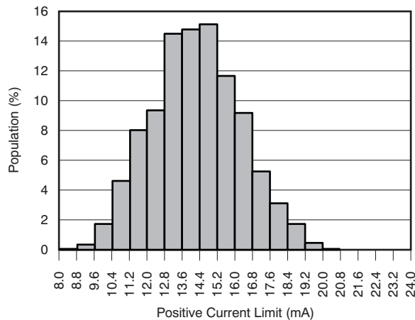
Figure 27. POSITIVE OUTPUT CURRENT LIMIT DISTRIBUTION
