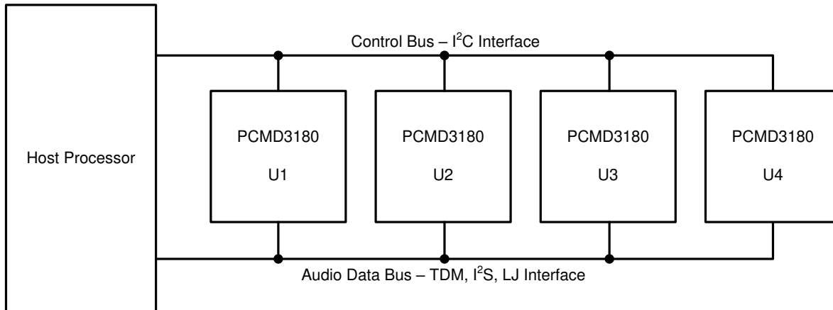
図 6-13. Multiple PCMD3180-Q1 Devices With Shared Control and Audio Data Buses
