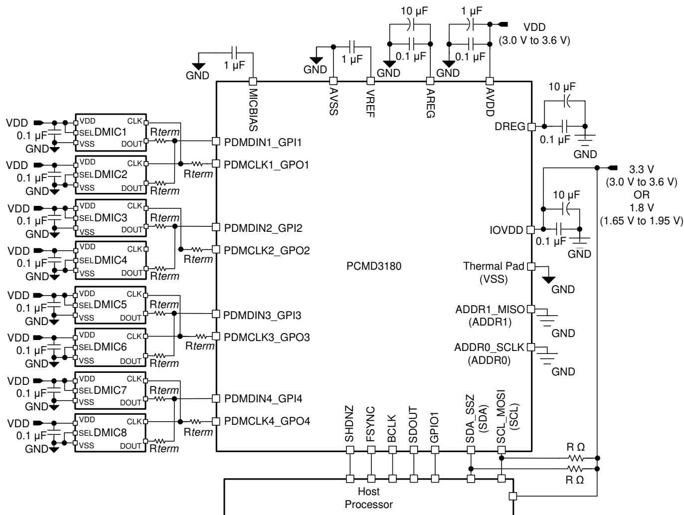
図 8-1. Eight-Channel Digital PDM Microphone Recording Diagram
