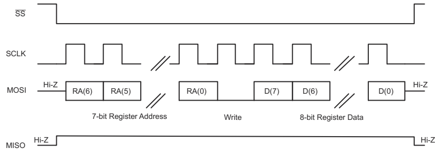
図 6-68. SPI Single-Byte Write Transfer
