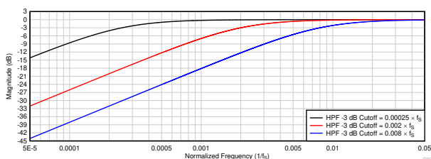
図 6-17. HPF Filter Frequency Response Plot
