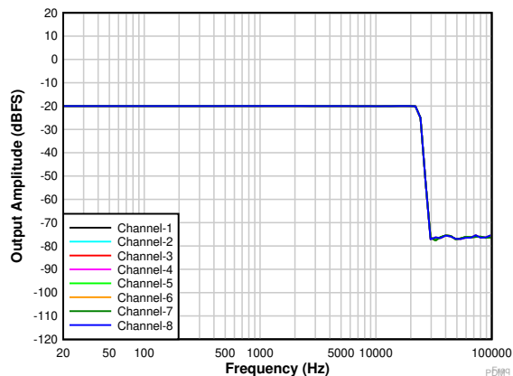
図 5-15. Frequency Response With a -20-dBr Input
