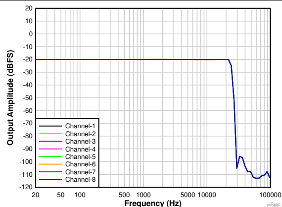
図 5-11. Frequency Response With a -20-dBr Input
