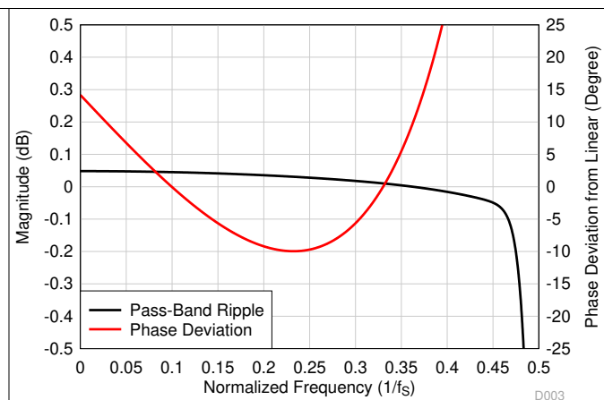
図 6-50. Ultra-Low-Latency Decimation Filter Pass-Band Ripple and Phase Deviation
