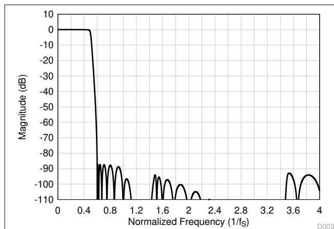
図 6-49. Ultra-Low-Latency Decimation Filter Magnitude Response
