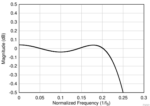
図 6-34. Linear Phase Decimation Filter Pass-Band Ripple
