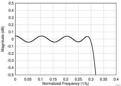
図 6-32. Linear Phase Decimation Filter Pass-Band Ripple
