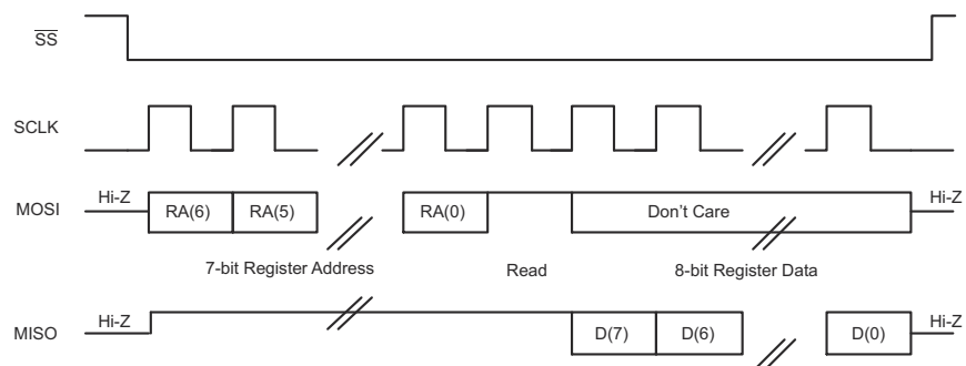
図 6-69. SPI Single-Byte Read Transfer
