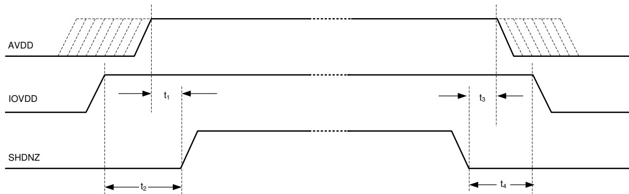
Figure 9-1. Power-Supply Sequencing Requirement Timing Diagram
