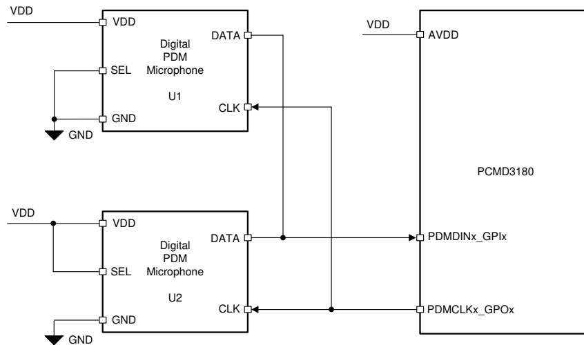
Figure 6-14. Digital PDM Microphones Connection Diagram to the PCMD3180-Q1
