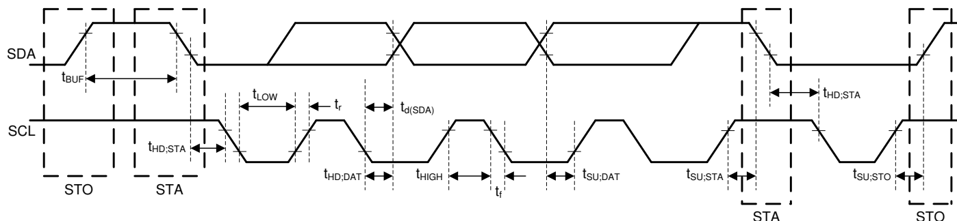
図 5-1. I 2 C Interface Timing Diagram
