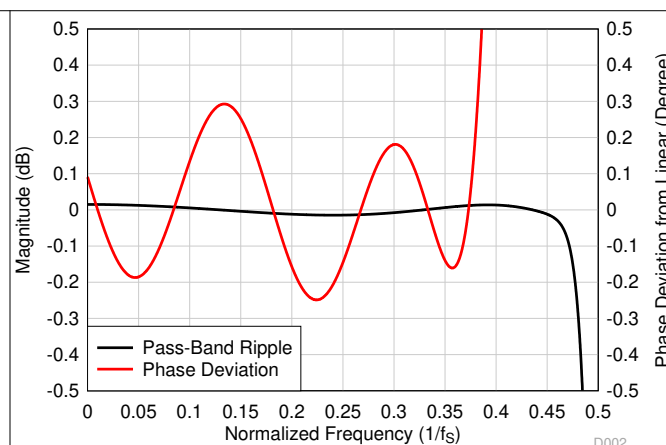
図 6-44. Low-Latency Decimation Filter Pass-Band Ripple and Phase Deviation
