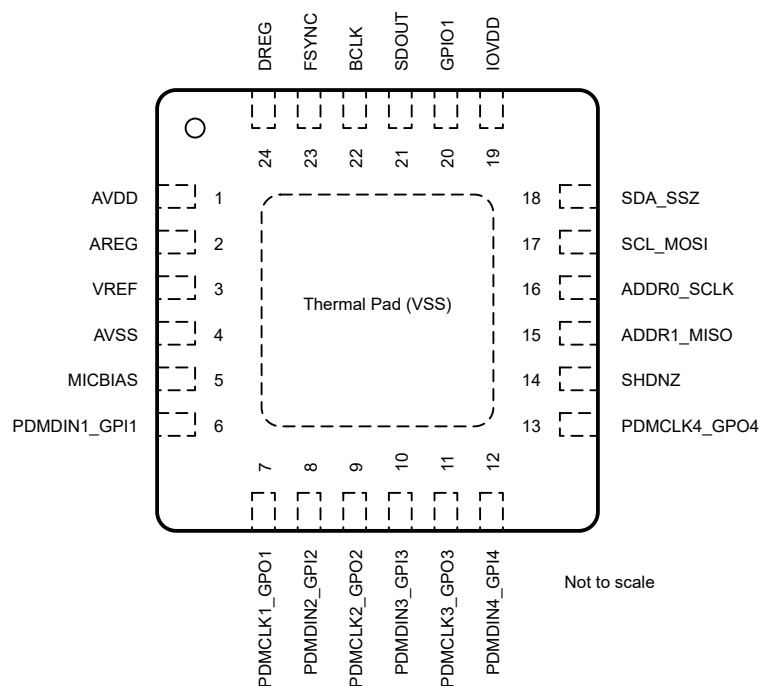
図 4-1. RTW Package 24-Pin WQFN With Exposed Thermal Pad Top View
