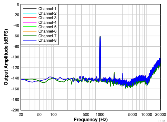
図 5-16. FFT With a -60-dBr Input
