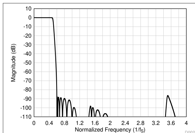
図 6-43. Low-Latency Decimation Filter Magnitude Response
