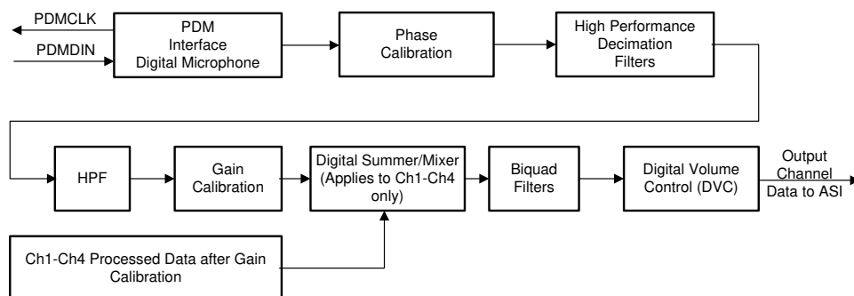
Figure 32. Signal-Chain Processing Flowchart
