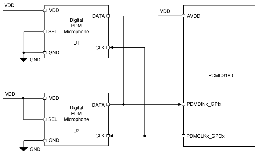
Figure 30. Digital PDM Microphones Connection Diagram to the PCMD3180
