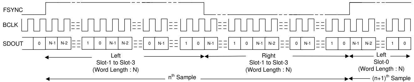
7-11. LJ Protocol Timing (No Idle BCLK Cycles, TX_OFFSET = 0)
