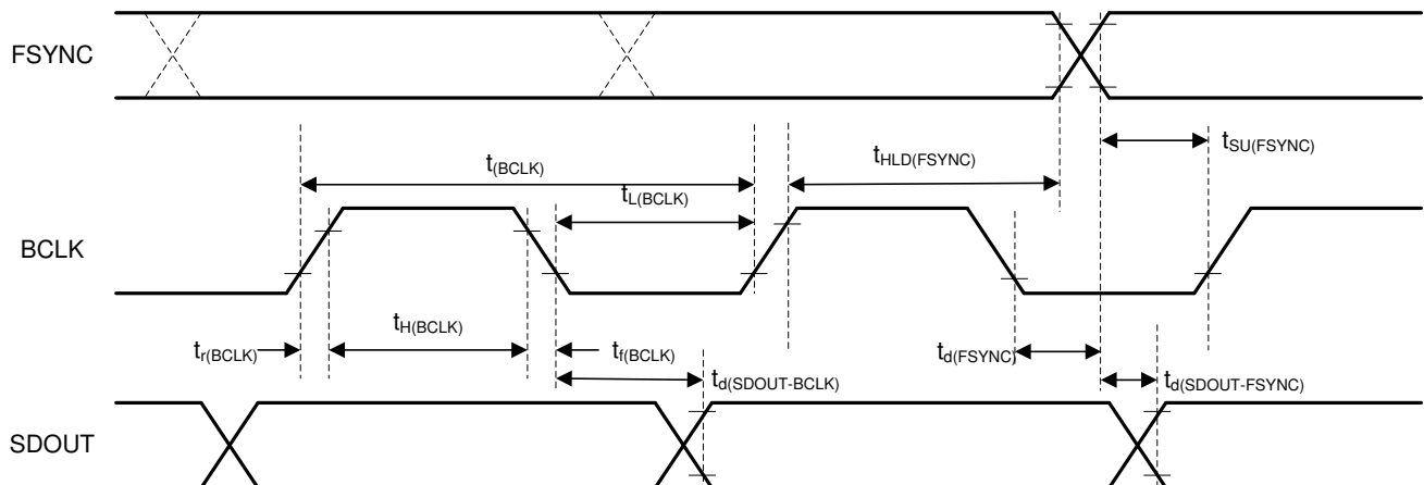
Figure 6-2. TDM (With BCLK_POL = 1), I²S, and LJ Interface Timing Diagram
