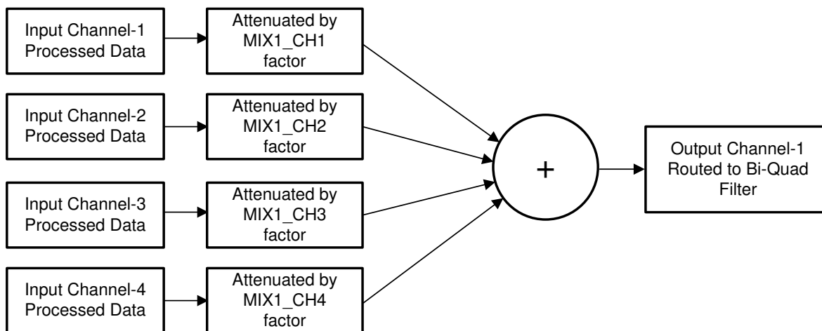
图 7-18. Programmable Digital Mixer Block Diagram
