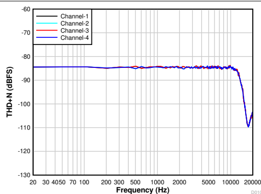
4th-order PDM modulator with PDMCLKx = 1.536\text{ MHz}
