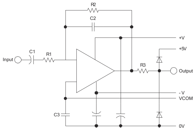
図 8-2. V_{COM} Biased Buffering Example
