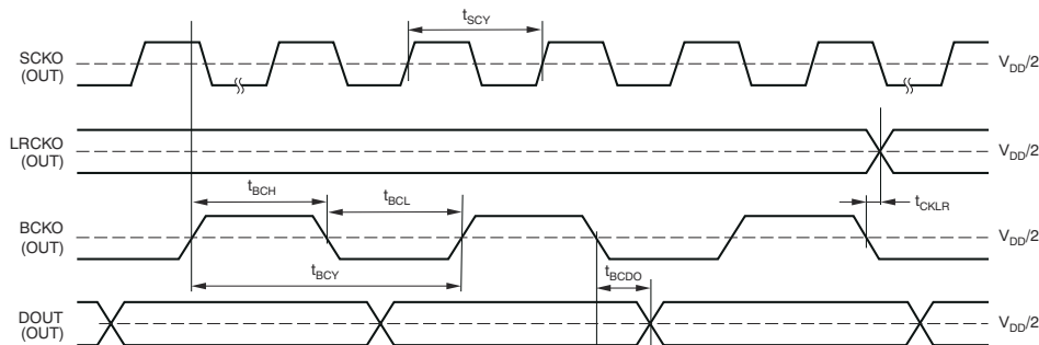
FIG 7-13. DIR Decoded Audio Data Output Timing
