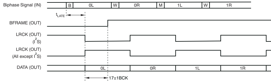
FIG 7-12. Latency Time Between Input Biphase and LRCKO/DOUT
