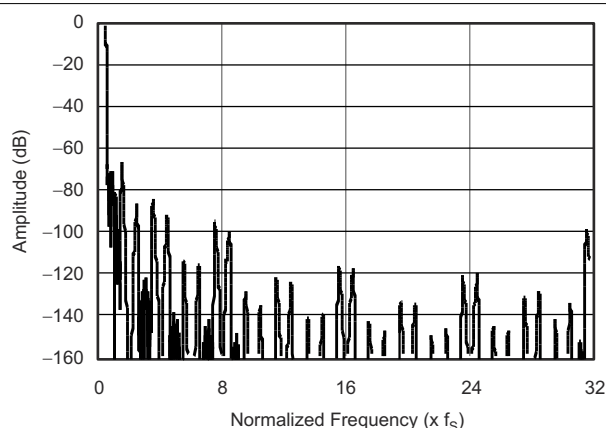
6-5. Decimation Filter Stop Band Characteristic
