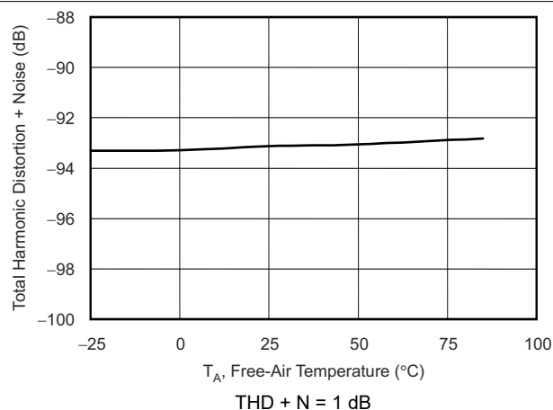
FIG 6-1. Total Harmonic Distortion + Noise vs Temperature
