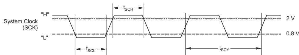
図 7-3. ADC System Clock Input Timing
