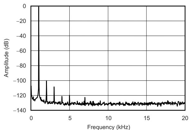
8-4. Output Spectrum
