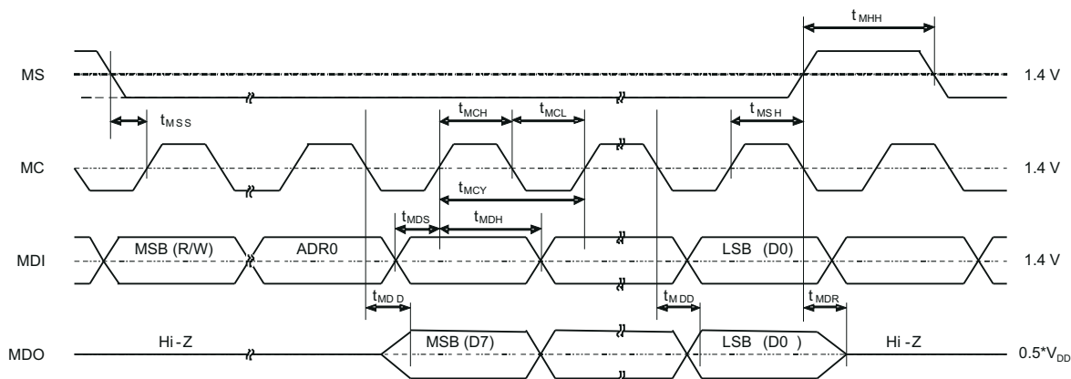
7-29. Control Interface Timing Requirements
