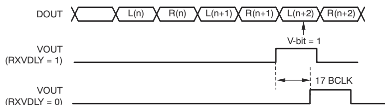
FIG 7-15. RXVDLY and VOUT Timing
