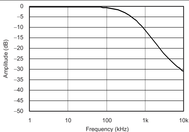
6-8. Antialiasing Filter Characteristic
