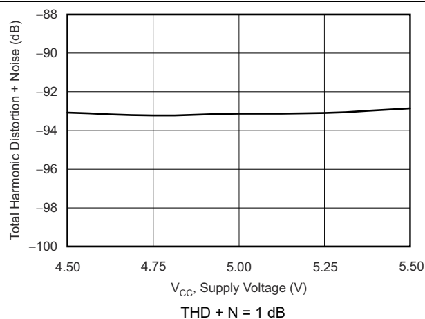
FIG 6-3. Total Harmonic Distortion + Noise vs Supply Voltage
