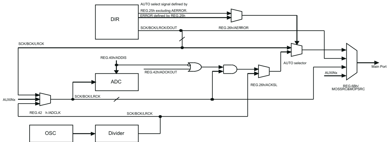
FIG 7-21. Clock Tree Diagram for Auto Source Selector
