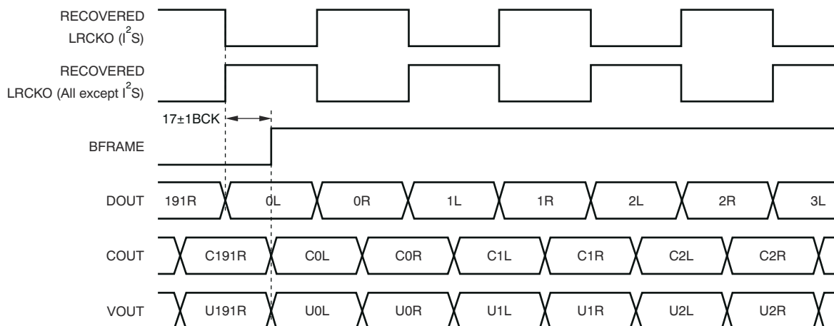
FIG 7-14. LRCKO, DOUT, BFRAME, COUT, UOUT, and VOUT Output Timing
