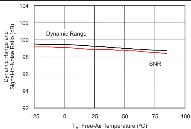
FIG 6-2. Dynamic Range and SNR vs Temperature
