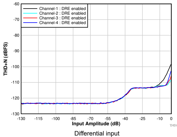
Figure 6-5. THD+N vs Input Amplitude With DRE Enabled
