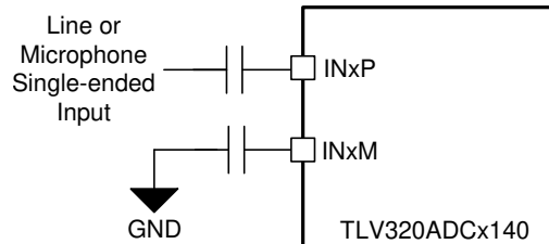
図 7-15. Single-Ended AC-Coupled Input Connection
