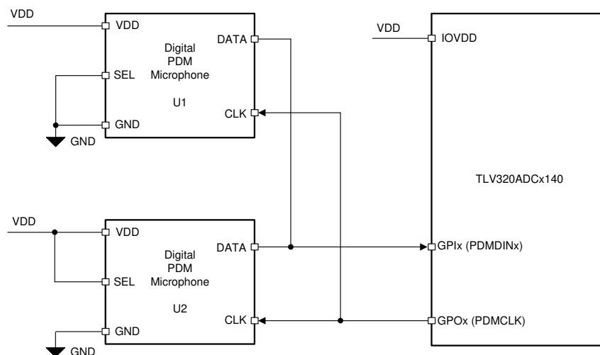
Figure 7-64. Digital PDM Microphones Connection Diagram to the PCM6140-Q1
