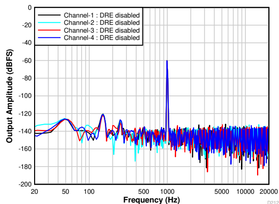
9-4. FFT With a -60-dBr Input With DRE Disabled
