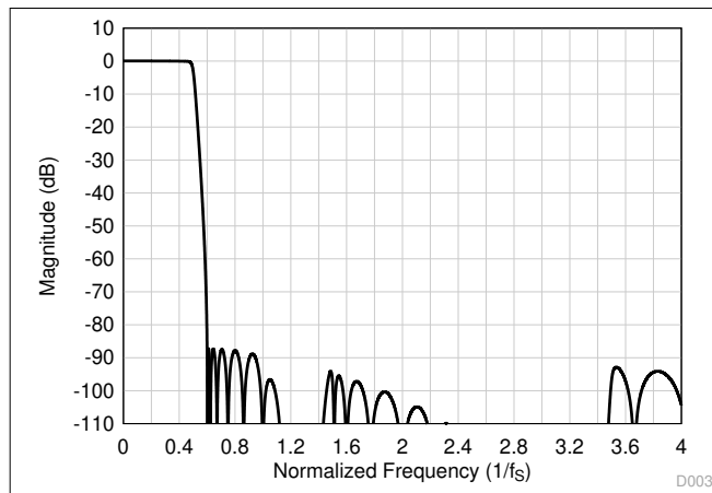
図 7-49. Ultra-Low-Latency Decimation Filter Magnitude Response
