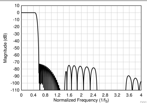
図 7-19. Linear Phase Decimation Filter Magnitude Response
