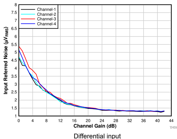
6-13. Input-Referred Noise vs Channel Gain
