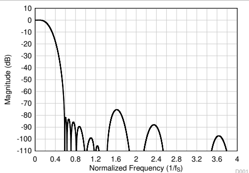
図 7-35. Linear Phase Decimation Filter Magnitude Response
