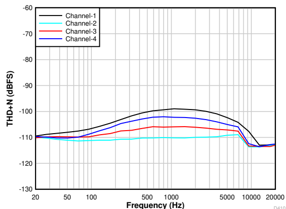
6-12. THD+N vs Input Frequency With a -1-dBr Input
