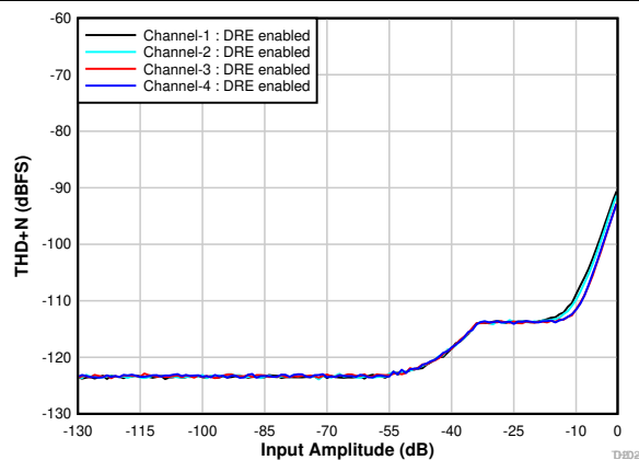
9-3. THD+N vs Input Amplitude With DRE Enabled
