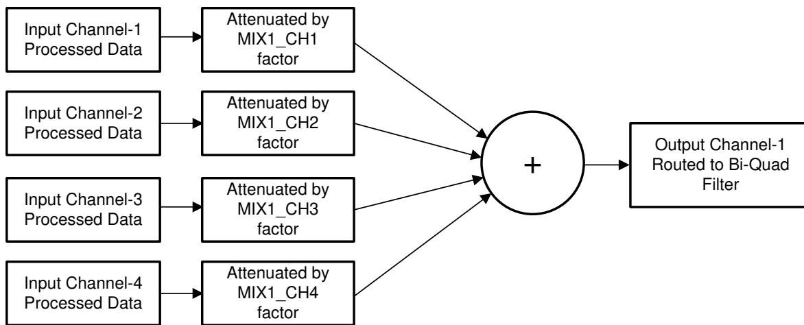
図 7-18. Programmable Digital Mixer Block Diagram
