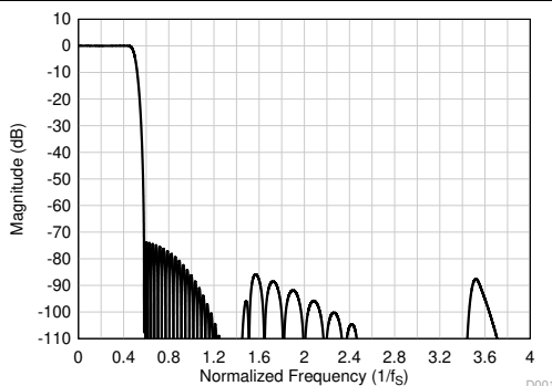
図 7-29. Linear Phase Decimation Filter Magnitude Response
