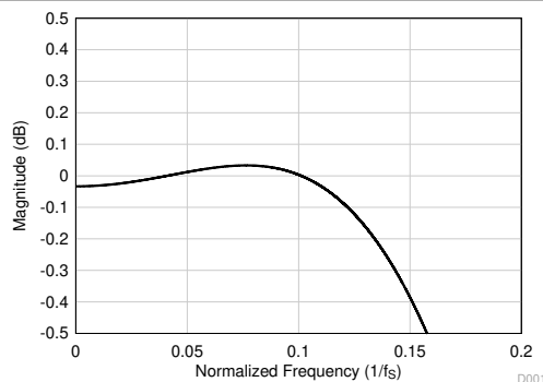
図 7-36. Linear Phase Decimation Filter Pass-Band Ripple
