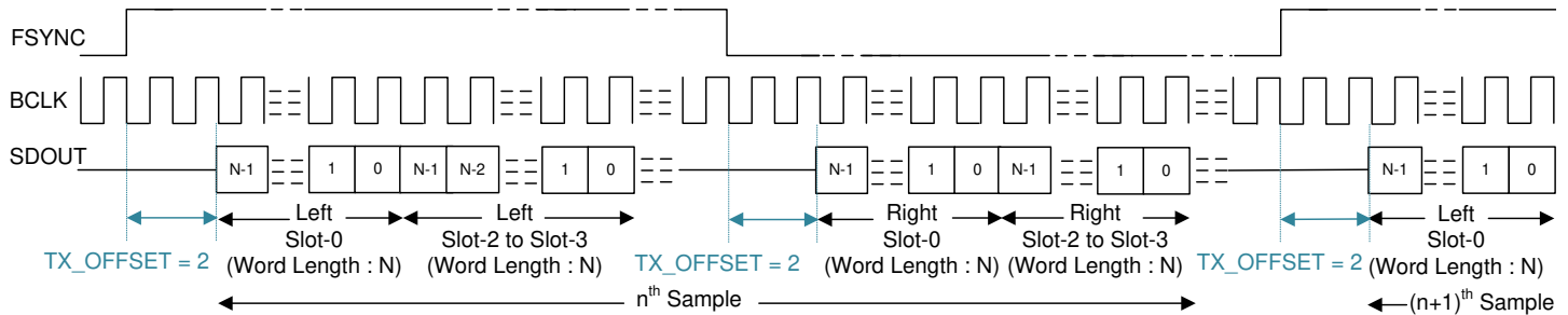
図 7-10. LJ Protocol Timing (TX_OFFSET = 2)
