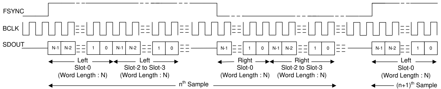
図 7-9. LJ Mode Standard Protocol Timing (TX_OFFSET = 0)
