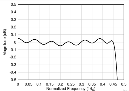
図 7-30. Linear Phase Decimation Filter Pass-Band Ripple
