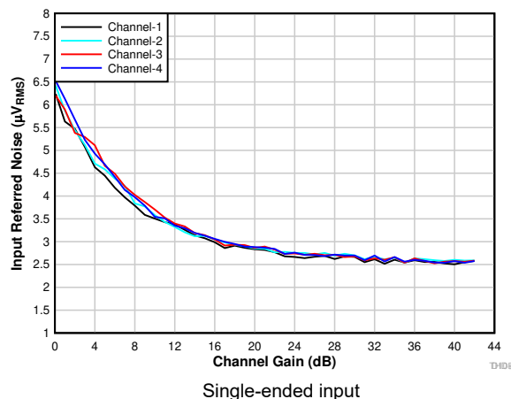
6-14. Input-Referred Noise vs Channel Gain
