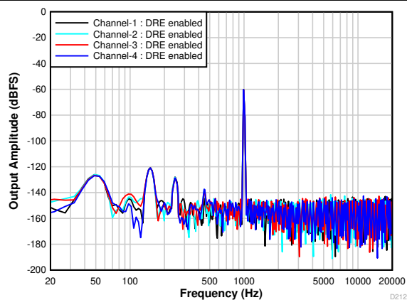
9-2. FFT With a -60-dBr Input With DRE Enabled
