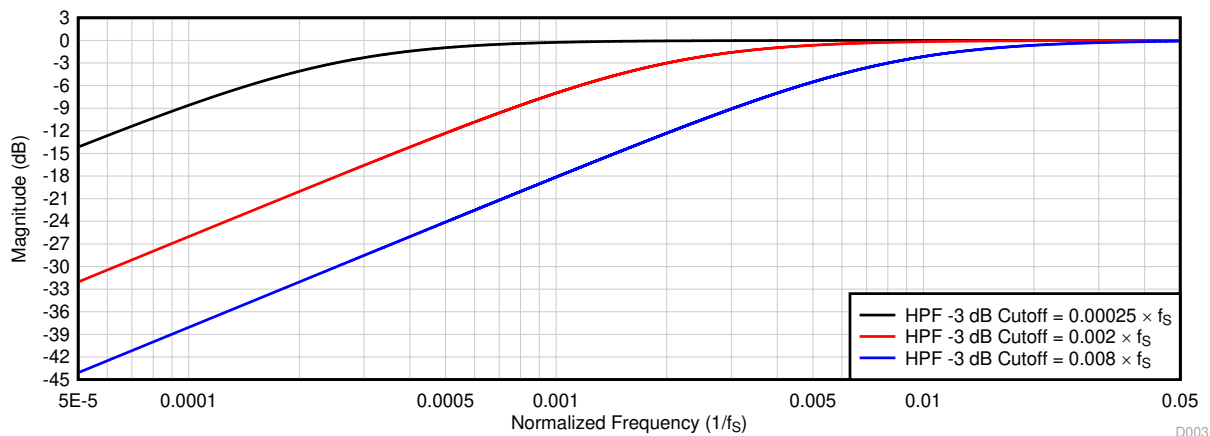
図 7-17. HPF Filter Frequency Response Plot
