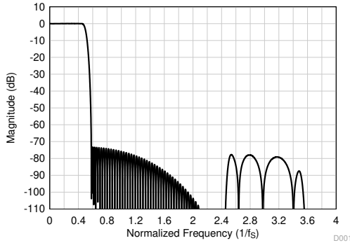
図 7-21. Linear Phase Decimation Filter Magnitude Response
