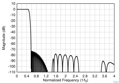
図 7-23. Linear Phase Decimation Filter Magnitude Response
