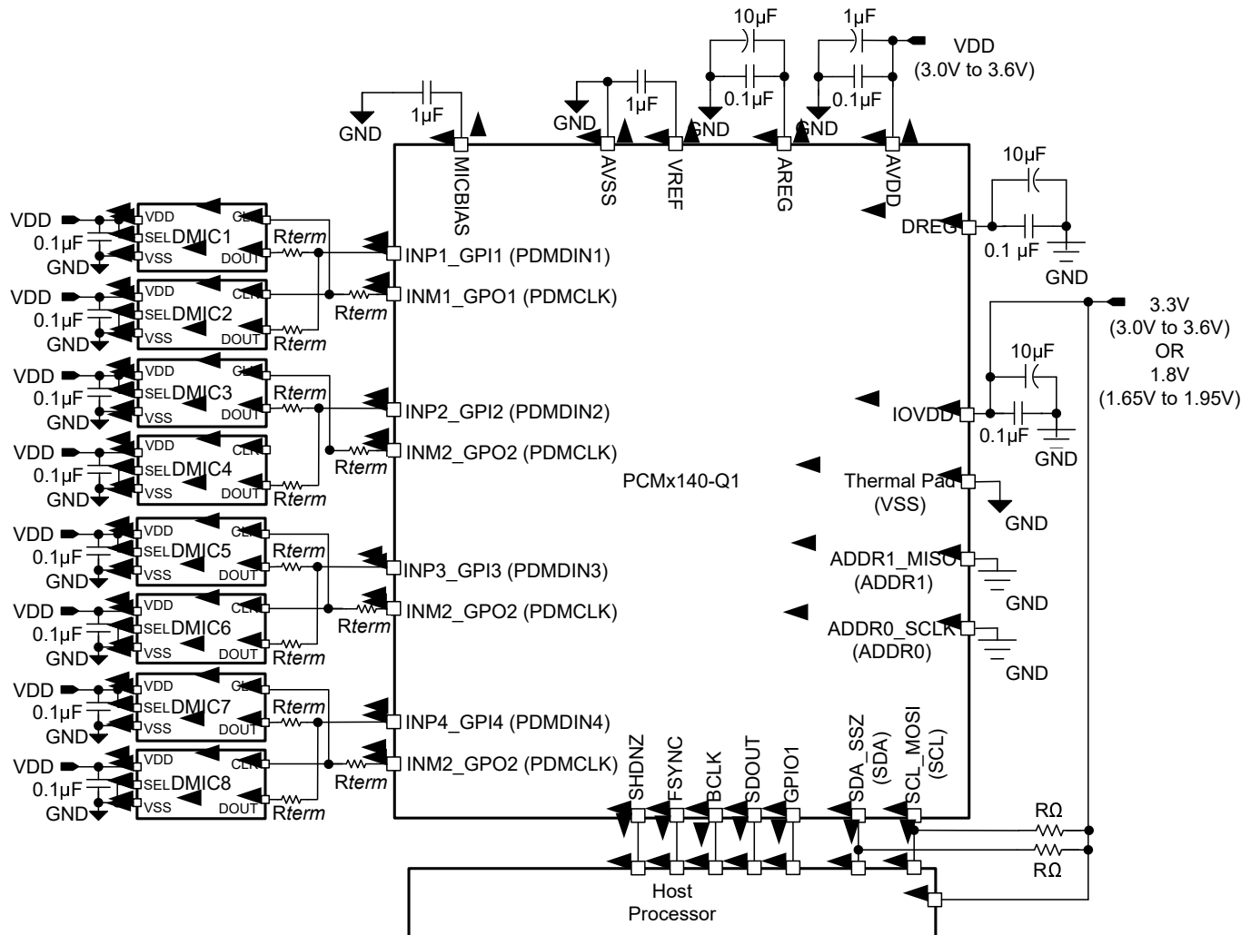
図 9-6. Eight-Channel Digital PDM Microphone Recording Diagram
