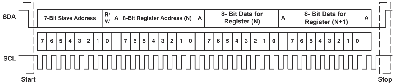
Figure 7-66. Typical I²C Sequence
