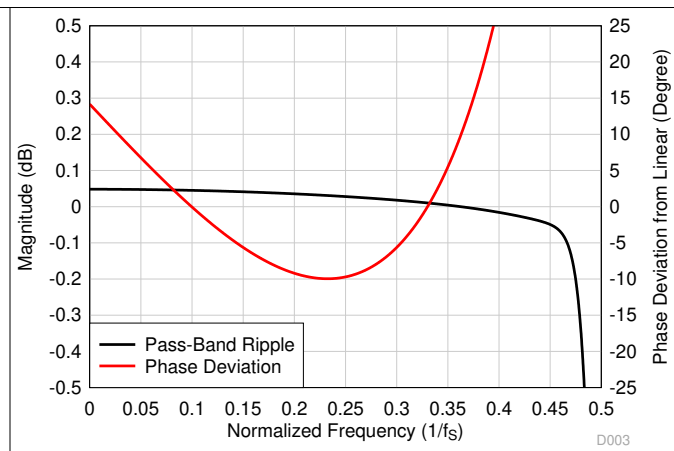
図 7-50. Ultra-Low-Latency Decimation Filter Pass-Band Ripple and Phase Deviation
