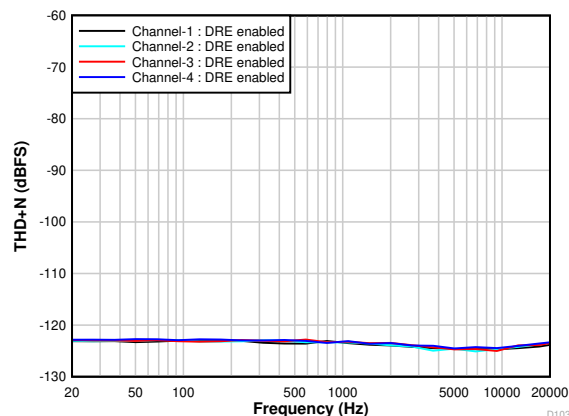
6-11. THD+N vs Input Frequency With a -60-dBr Input
