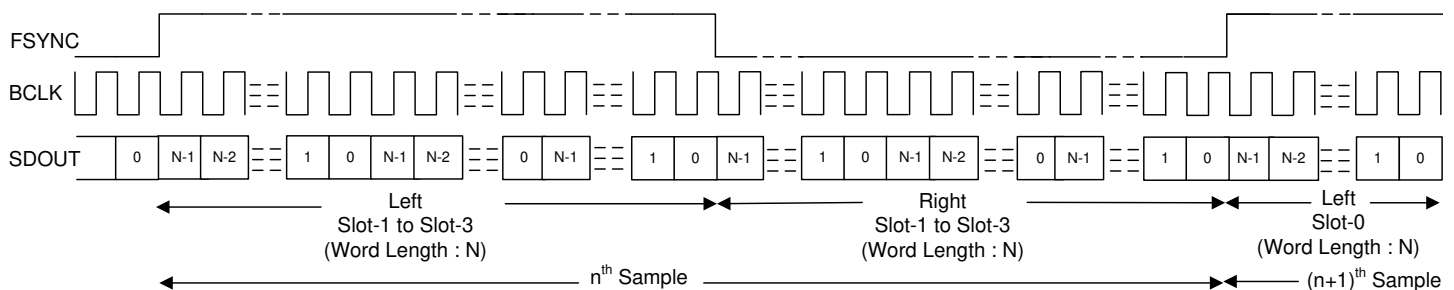
図 7-11. LJ Protocol Timing (No Idle BCLK Cycles, TX_OFFSET = 0)
