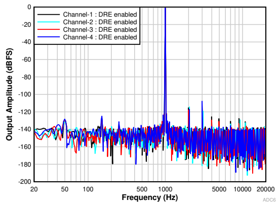
図 6-21. FFT With a -1-dBr Input With DRE Enabled
