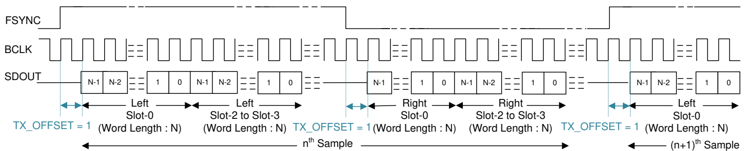
図 7-12. LJ Protocol Timing (TX_OFFSET = 1 and BCLK_POL = 1)
