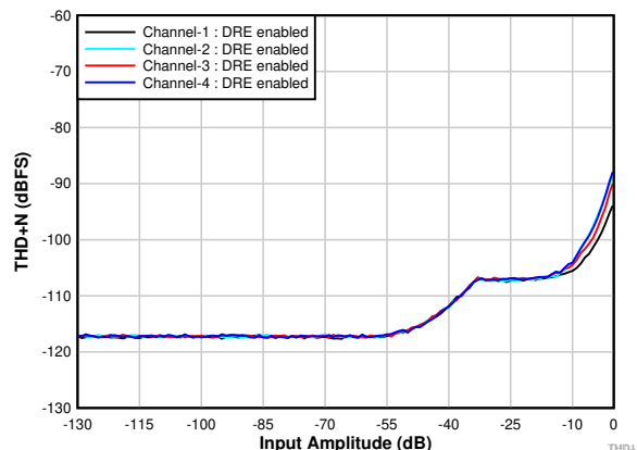
6-9. THD+N vs Input Amplitude With DRE Enabled
