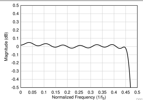
図 7-20. Linear Phase Decimation Filter Pass-Band Ripple
