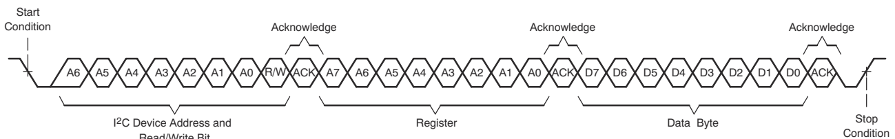
Figure 7-67. I²C Single-Byte Write Transfer
