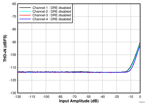
9-5. THD+N vs Input Amplitude With DRE Disabled
