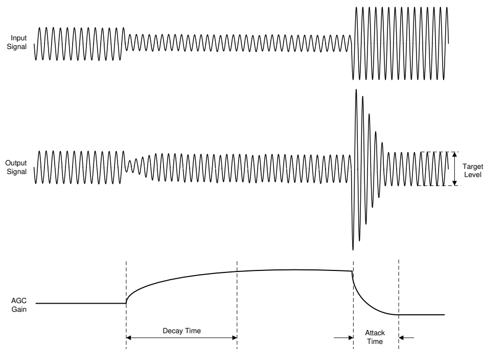
図 7-63. AGC Characteristics
