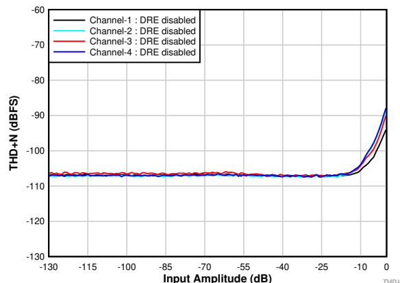
6-10. THD+N vs Input Amplitude With DRE Disabled
