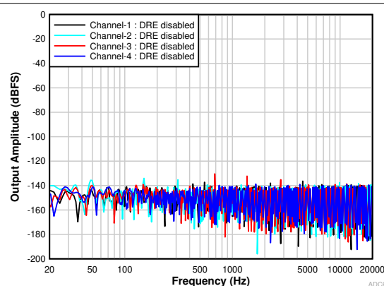
Figure 6-18. FFT With Idle Input With DRE Disabled
