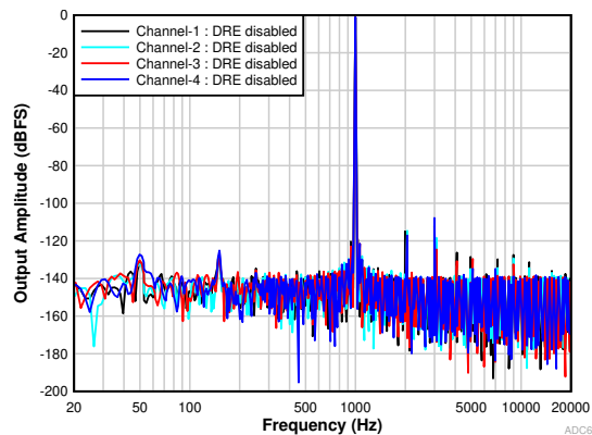
図 6-22. FFT With a -1-dBr Input With DRE Disabled
