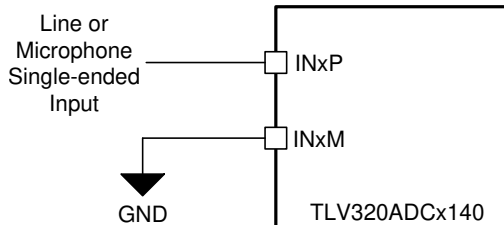
図 7-14. Single-Ended DC-Coupled Input Connection
