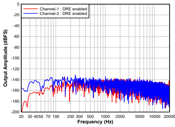
FIG 7-21. Single Ended FFT With Idle Input With DRE Enabled
