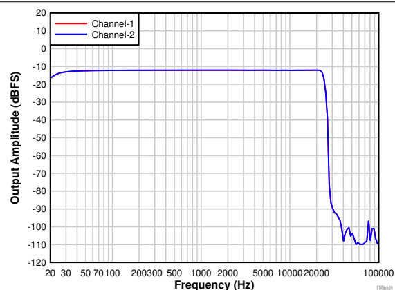
7-15. Frequency Response With a -12-dBr Input
