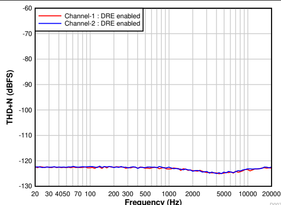
7-10. THD+N vs Input Frequency at -60-dBr Input With DRE Enabled
