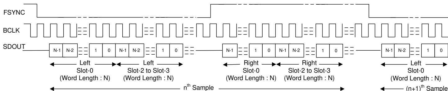
8-8. I 2 S Protocol Timing (TX_OFFSET = 0 and BCLK_POL = 1)
