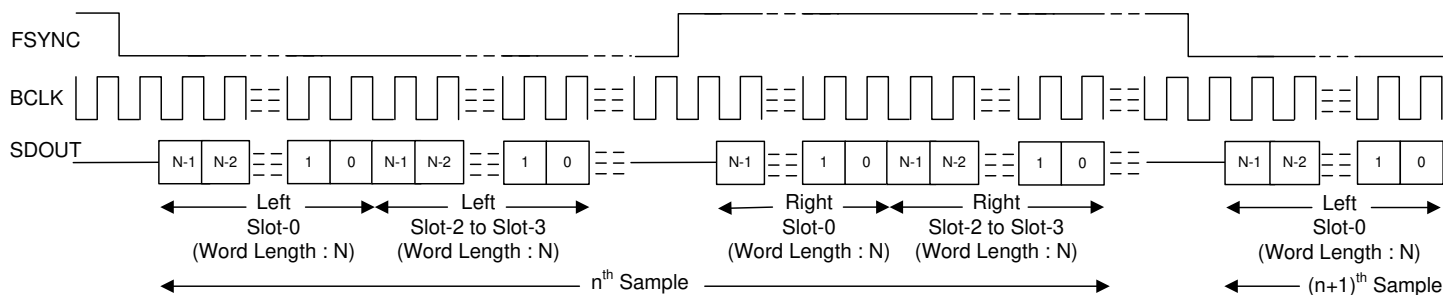
8-5. I 2 S Mode Standard Protocol Timing (TX_OFFSET = 0)
