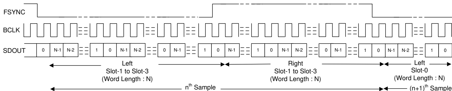
8-7. I 2 S Protocol Timing (No Idle BCLK Cycles, TX_OFFSET = 0)
