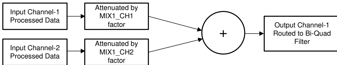
图 8-20. Programmable Digital Mixer Block Diagram
