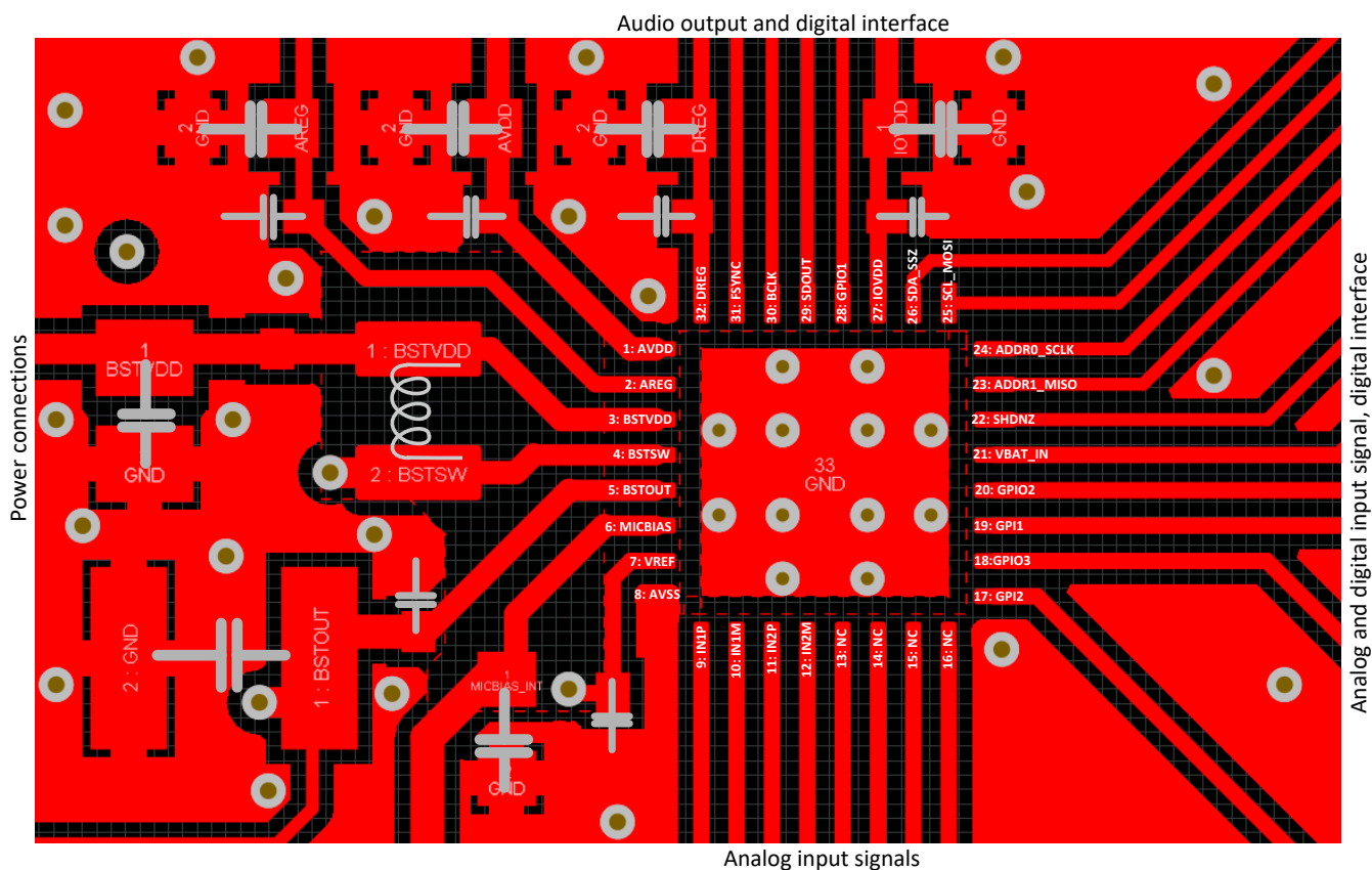
11-1. Layout Example of the PCM6020-Q1
