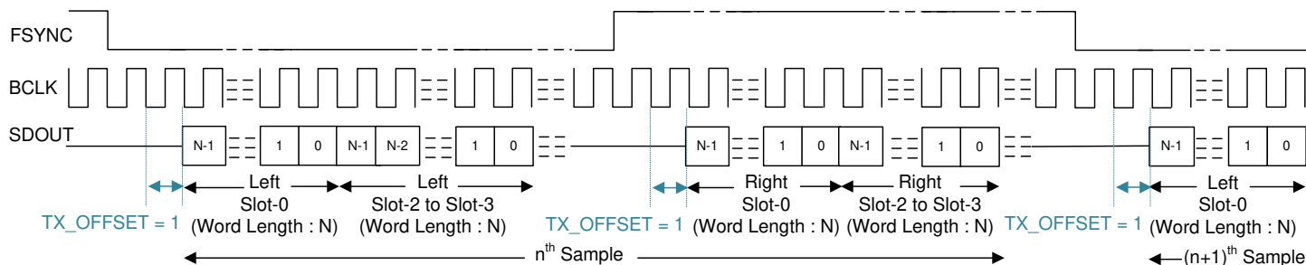
8-6. I 2 S Protocol Timing (TX_OFFSET = 1)
