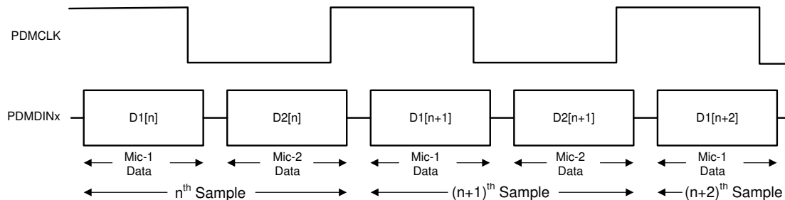
7-65. Digital PDM Microphone Protocol Timing Diagram
