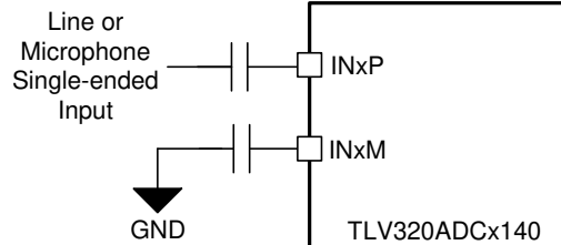
図 7-15. Single-Ended AC-Coupled Input Connection
