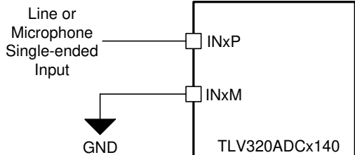
図 7-14. Single-Ended DC-Coupled Input Connection
