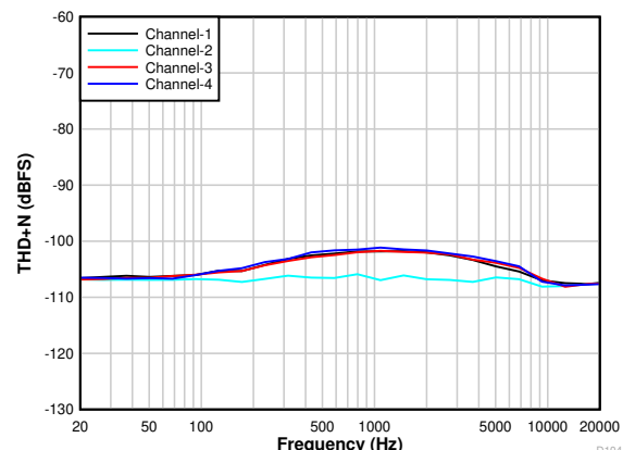
6-12. THD+N vs Input Frequency With a -1-dBr Input
