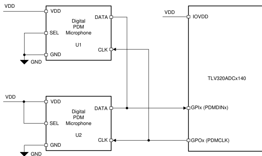
7-64. Digital PDM Microphones Connection Diagram to the PCM5140-Q1
