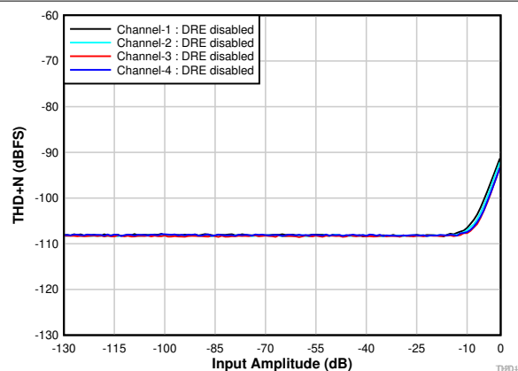
8-5. THD+N vs Input Amplitude With DRE Disabled
