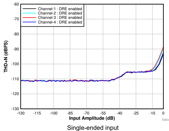
6-7. THD+N vs Input Amplitude With DRE Enabled
