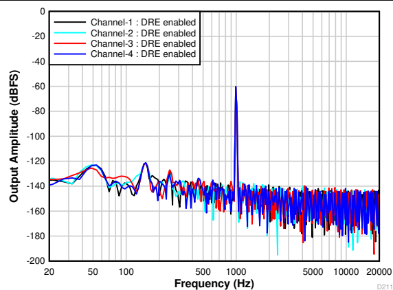
8-2. FFT With a -60-dBr Input With DRE Enabled
