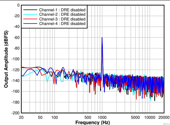
8-4. FFT With a -60-dBr Input With DRE Disabled
