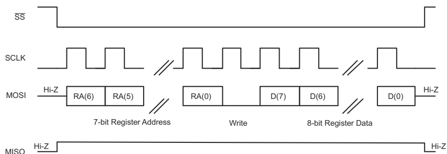
図 7-71. SPI Single-Byte Write Transfer
