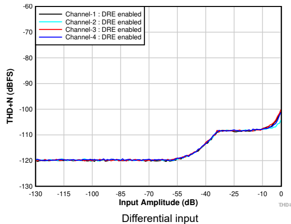
6-5. THD+N vs Input Amplitude With DRE Enabled
