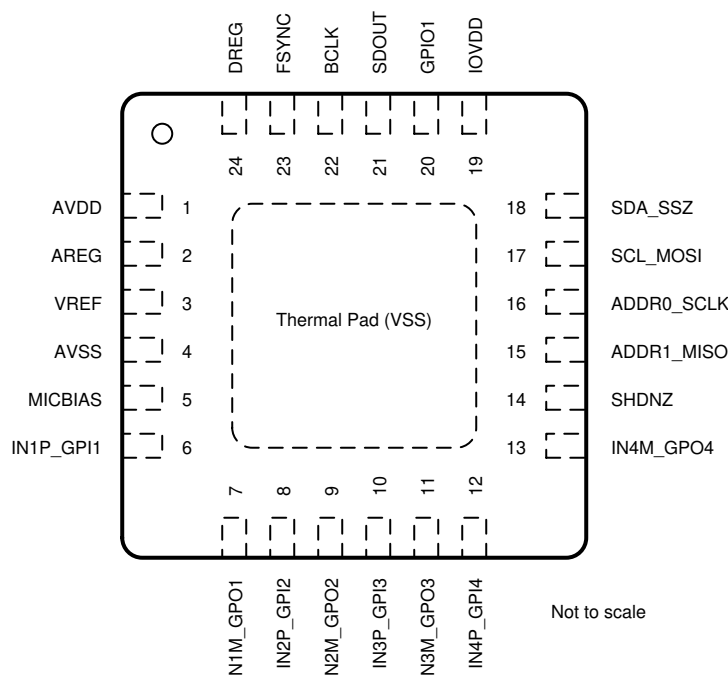
図 5-1. RTW Package 24-Pin WQFN With Exposed Thermal Pad Top View
