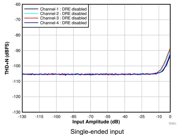
6-8. THD+N vs Input Amplitude With DRE Disabled
