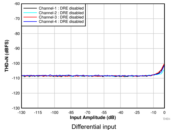
6-6. THD+N vs Input Amplitude With DRE Disabled
