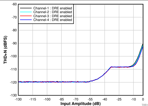
8-3. THD+N vs Input Amplitude With DRE Enabled
