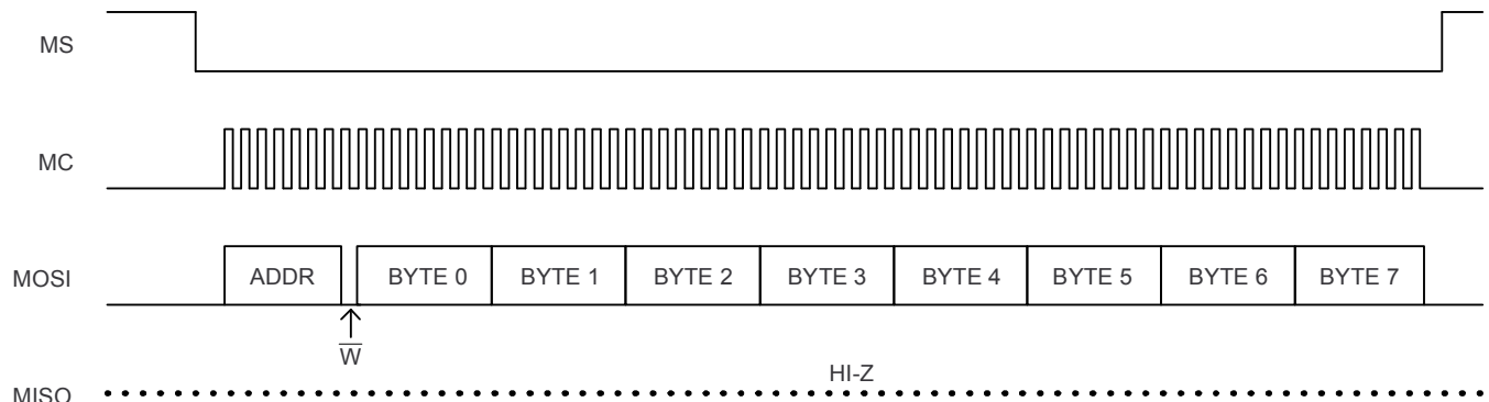
Figure 68. Serial Control Format; Write, Multiple Byte
