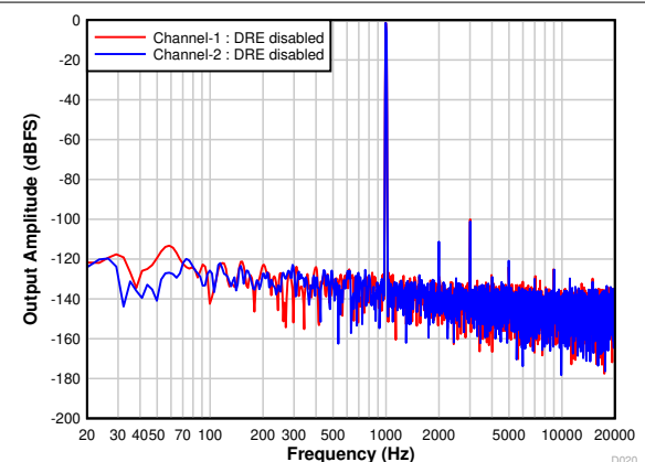
7-27. Differential FFT With a -1\text{-dBr} Input With DRE Disabled
