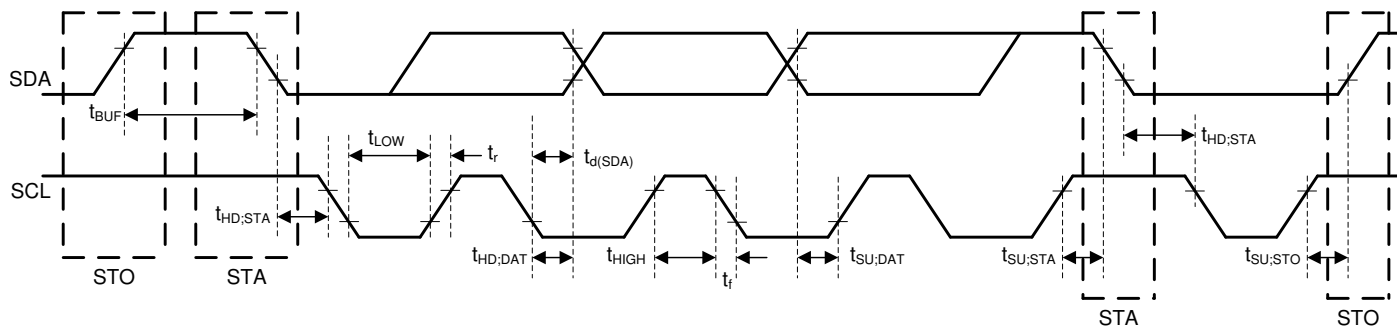
Figure 7-1. I²C Interface Timing Diagram
