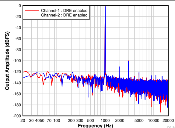
7-26. Differential FFT With a -1\text{-dBr} Input With DRE Enabled
