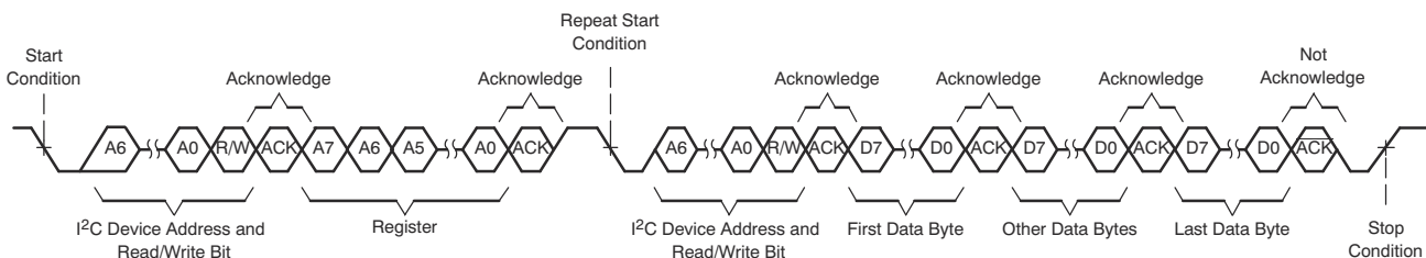
❏ 8-70. I 2 C Multiple-Byte Read Transfer
