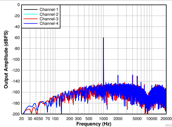
7-30. PDM Input FFT With a -60\text{-dBr} Input
