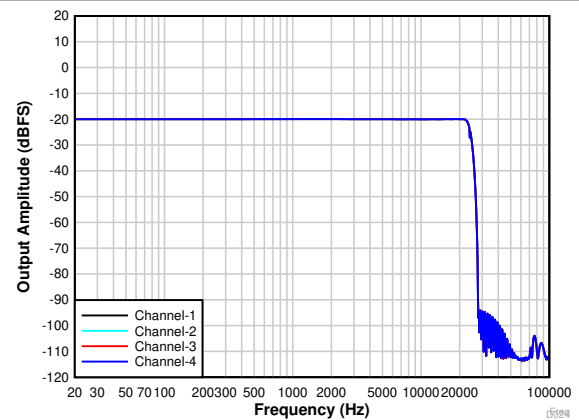
7-31. PDM Input Frequency Response With a -20\text{-dBr} Input
