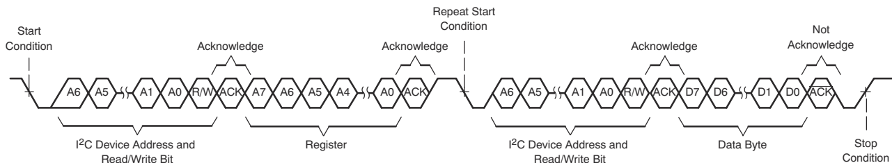
❏ 8-69. I 2 C Single-Byte Read Transfer
