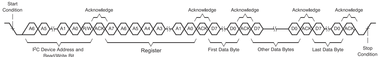
❏ 8-68. I 2 C Multiple-Byte Write Transfer
