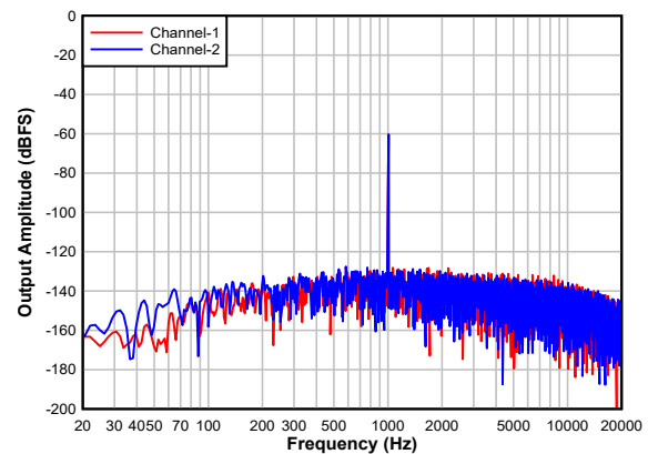
7-25. Single Ended FFT With a -60\text{-dBr} Input With DRE Disabled
