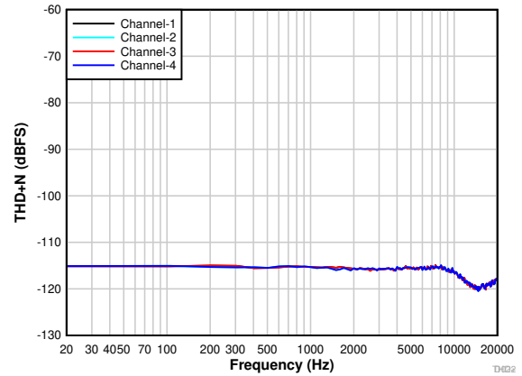
7-29. PDM Input THD+N vs Input Frequency With a -20\text{-dBr} Input
