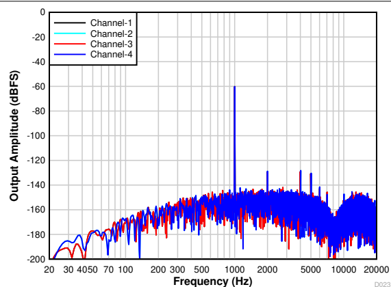
7-30. PDM Input FFT With a -60-dBr Input
