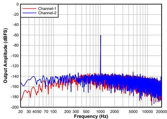
7-24. Single Ended FFT With a -60\text{-dBr} Input With DRE Enabled
