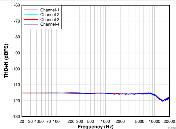
7-29. PDM Input THD+N vs Input Frequency With a -20-dBr Input
