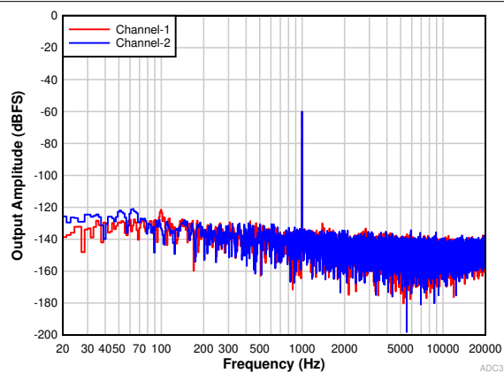
9-2. FFT With a -60-dBr Input
