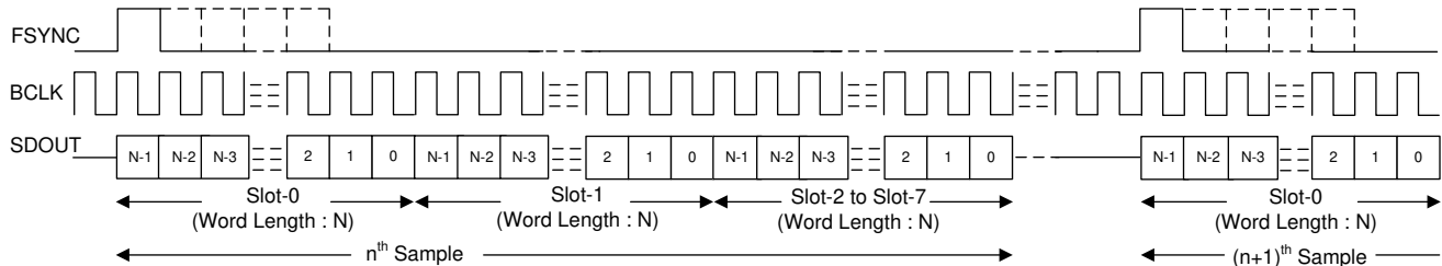
図 8-1. TDM Mode Standard Protocol Timing (TX_OFFSET = 0)
