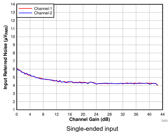
7-10. Input-Referred Noise vs Channel Gain
