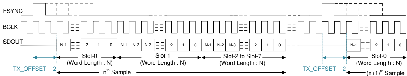
図 8-2. TDM Mode Protocol Timing (TX_OFFSET = 2)
