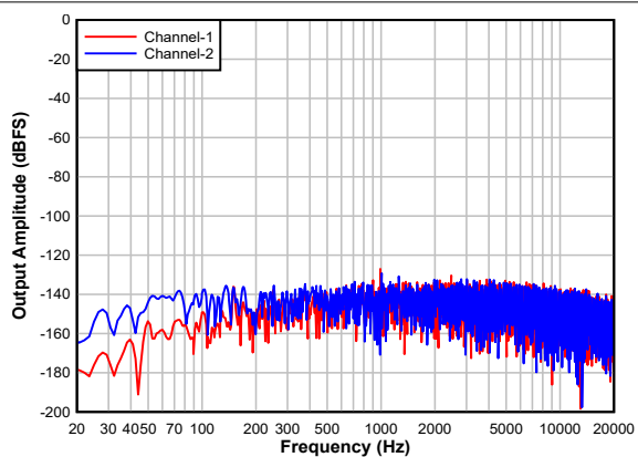
7-15. Single Ended FFT With Idle Input
