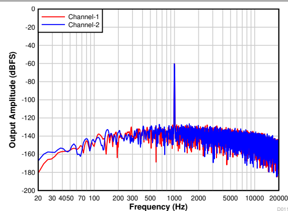
7-14. Differential FFT With a -60-dBr Input
