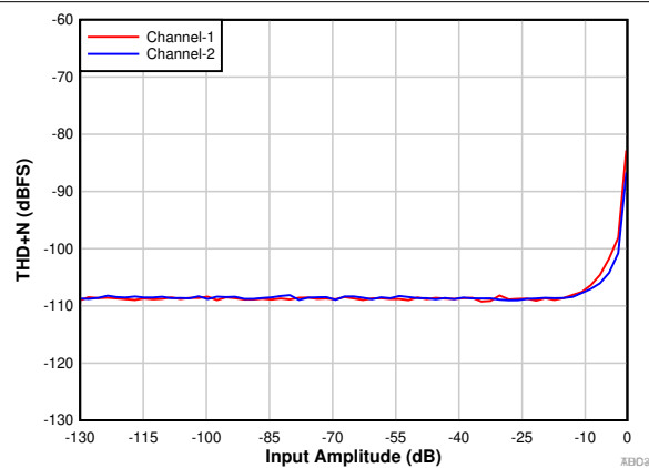
9-3. THD+N vs Input Amplitude
