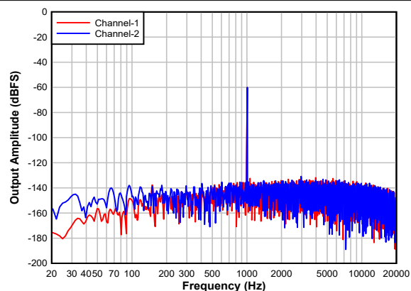
7-16. Single Ended FFT With a -60-dBr Input
