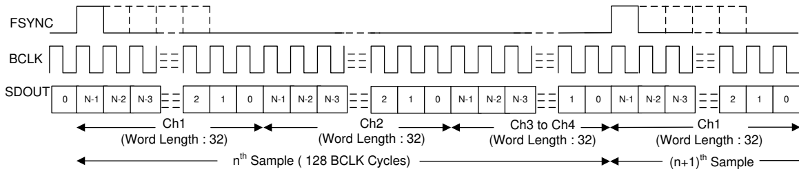
FIG 8-3. TDM Mode Protocol Timing (FMT0 = LOW) In Master Mode
