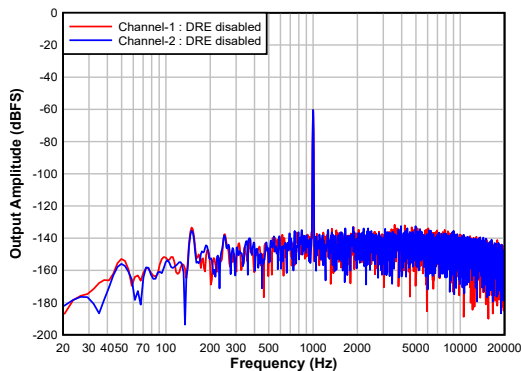
FIG 7-11. Differential Input: FFT With a -60\text{-dBr} Input and DRE Disabled
