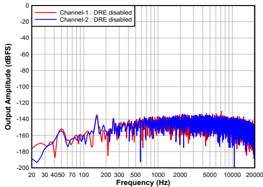
FIG 7-9. Differential Input: FFT With Idle Input and DRE Disabled
