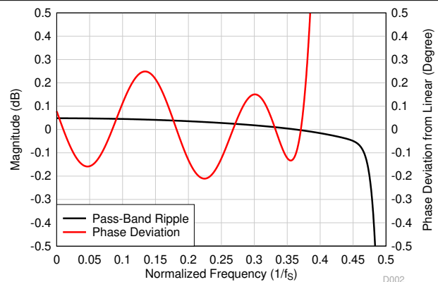
Figure 8-24. Low-Latency Decimation Filter Pass-Band Ripple and Phase Deviation
