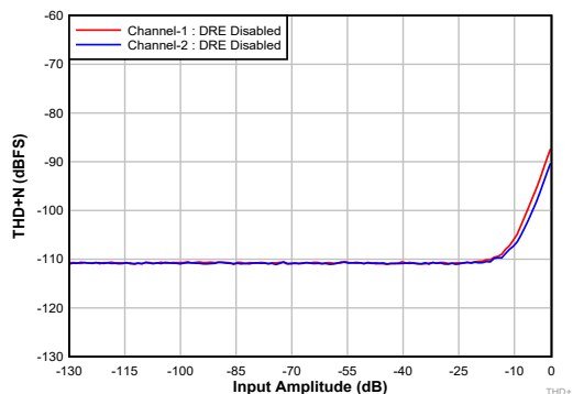
7-13. Single-Ended Input: THD+N vs Input Amplitude With DRE Disabled
