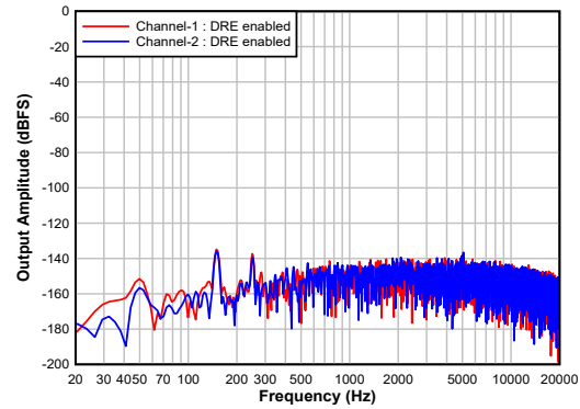
FIG 7-8. Differential Input: FFT With Idle Input and DRE Enabled
