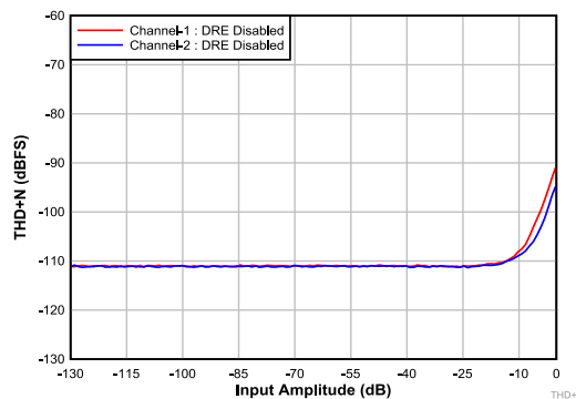
FIG 7-2. Differential Input: THD+N vs Input Amplitude With DRE Disabled
