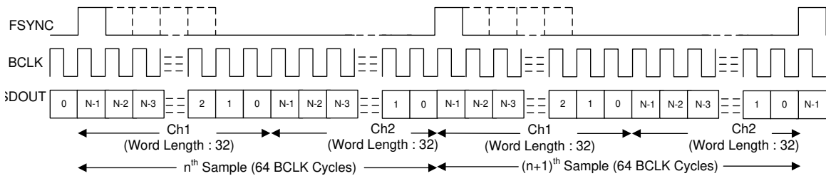
FIG 8-4. TDM Mode Protocol Timing (FMT0 = HIGH) In Master Mode
