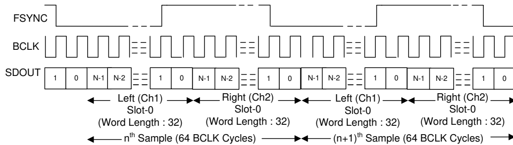
图 8-6. I 2 S Protocol Timing In Master Mode
