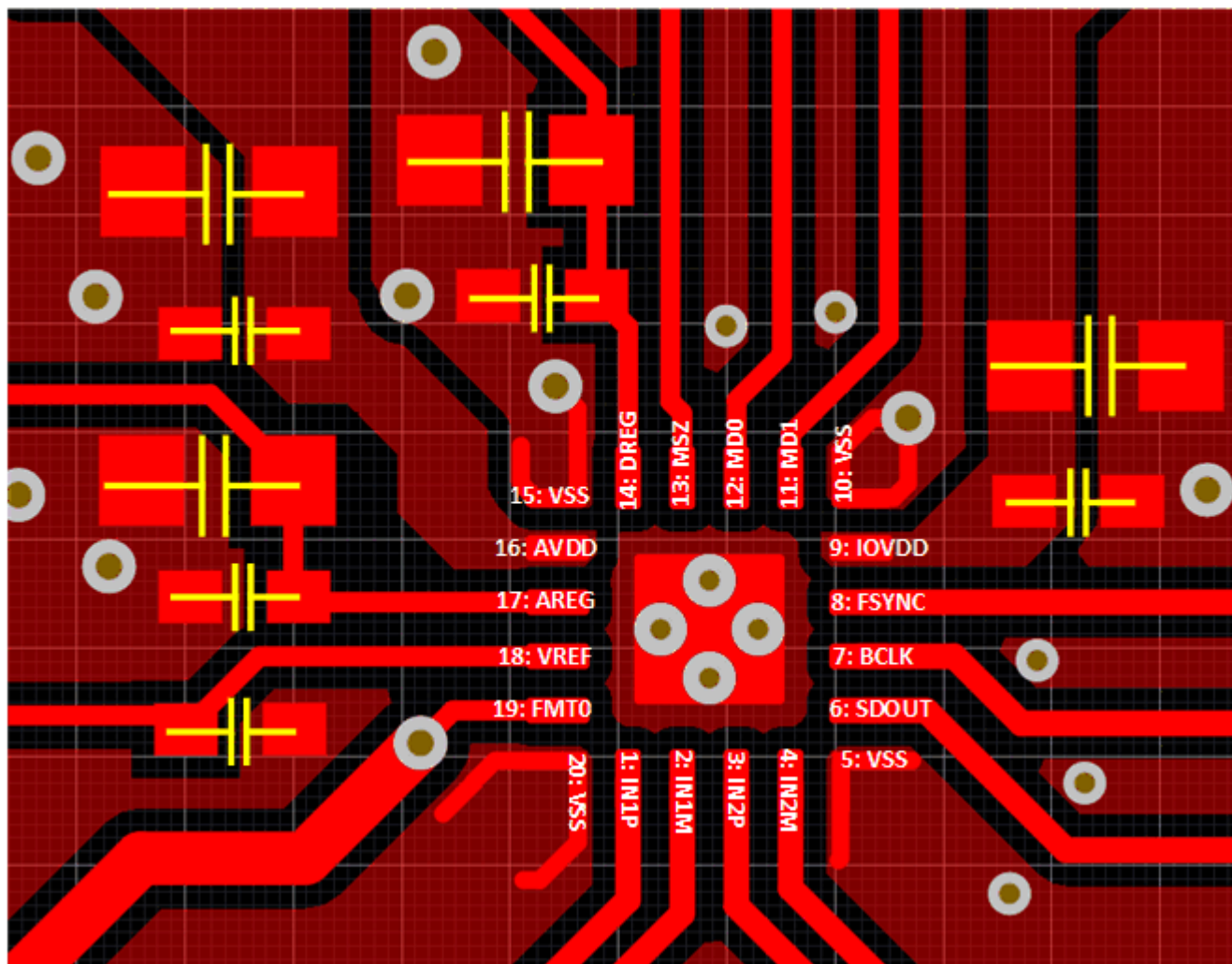
✎ 11-1. Example Layout
