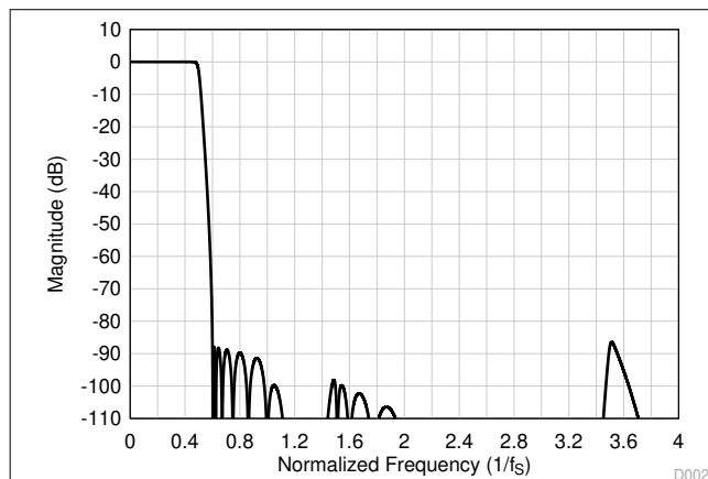
图 8-29. Low-Latency Decimation Filter Magnitude Response
