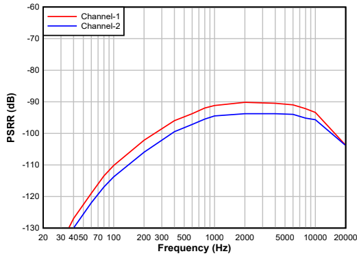
FIG 7-7. Power-Supply Rejection Ratio vs Ripple Frequency With a 100-mV PP Amplitude
