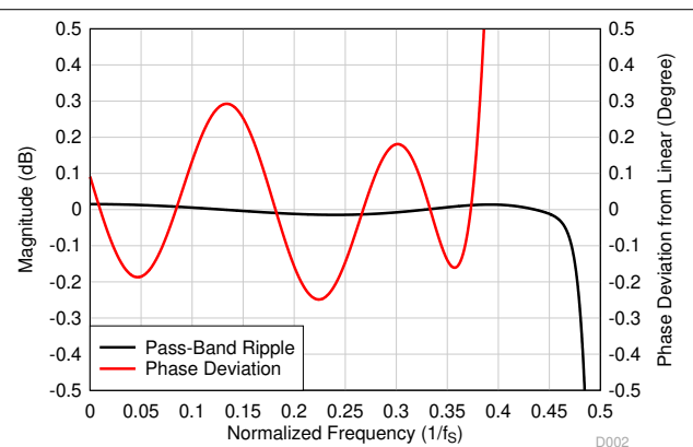
图 8-30. Low-Latency Decimation Filter Pass-Band Ripple and Phase Deviation
