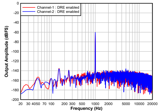
FIG 7-10. Differential Input: FFT With a -60\text{-dBr} Input and DRE Enabled
