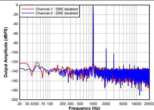
Figure 7-22. Single-ended Input: FFT With a -1\text{-dBr} Input
