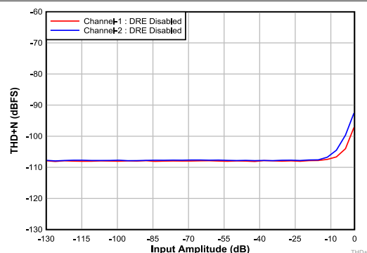
9-5. THD+N vs Input Amplitude With DRE Disabled
