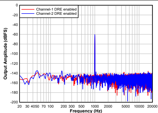
9-2. FFT With a –60-dBr Input With DRE Enabled
