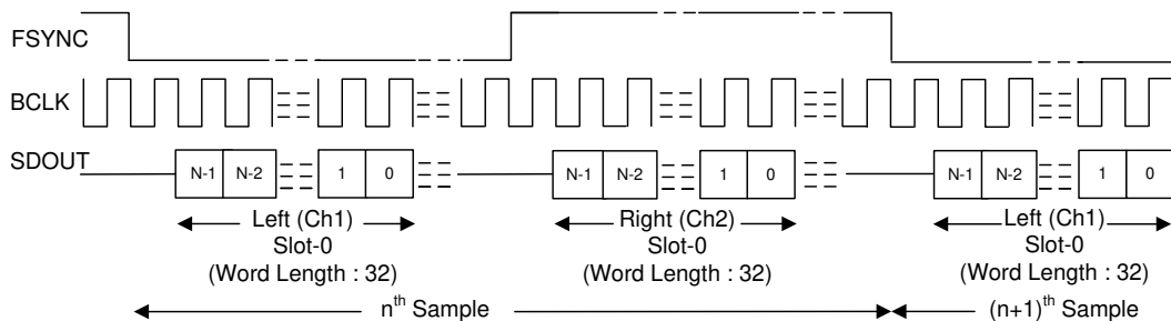
FIG 8-5. I 2 S Mode Protocol Timing in Slave Mode
