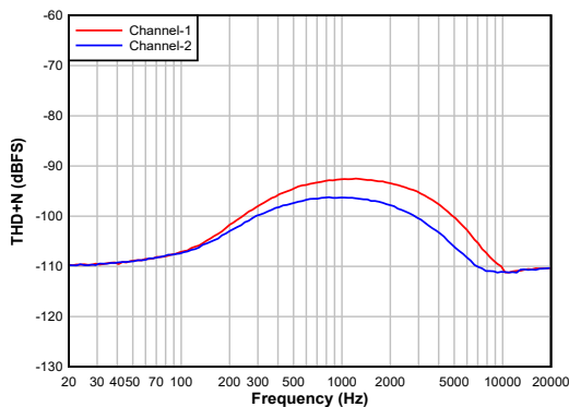
FIG 7-5. Differential Input: THD+N vs Input Frequency With a -1-dBr Input
