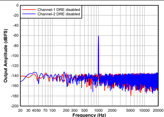
9-4. FFT With a –60-dBr Input With DRE Disabled
