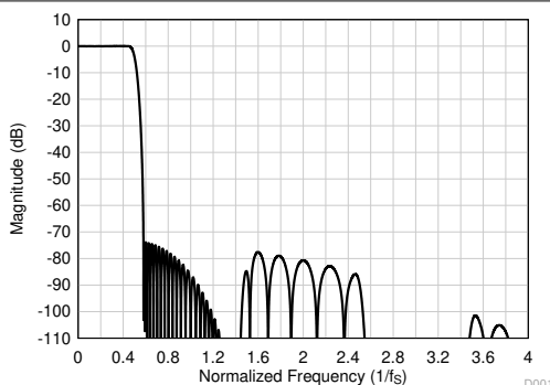
図 8-15. Linear Phase Decimation Filter Magnitude Response
