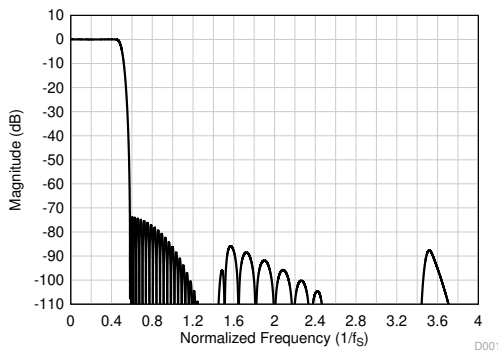
図 8-19. Linear Phase Decimation Filter Magnitude Response
