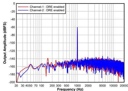
FIG 7-20. Single-ended Input: FFT With a -60\text{-dBr} Input and DRE Enabled
