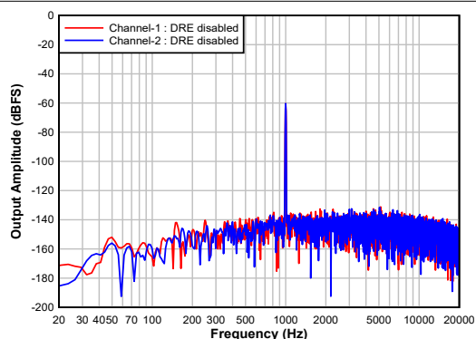
FIG 7-21. Single-ended Input: FFT With a -60\text{-dBr} Input and DRE Disabled
