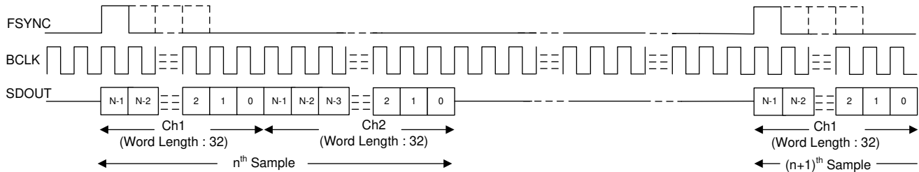
FIG 8-2. TDM Mode Protocol Timing (FMT0 = HIGH) In Slave Mode
