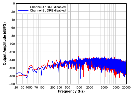
FIG 7-19. Single-ended Input: FFT With Idle Input and DRE Disabled
