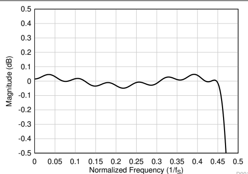
図 8-18. Linear Phase Decimation Filter Pass-Band Ripple
