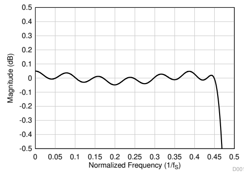
図 8-20. Linear Phase Decimation Filter Pass-Band Ripple
