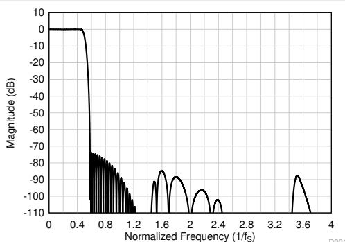
図 8-17. Linear Phase Decimation Filter Magnitude Response
