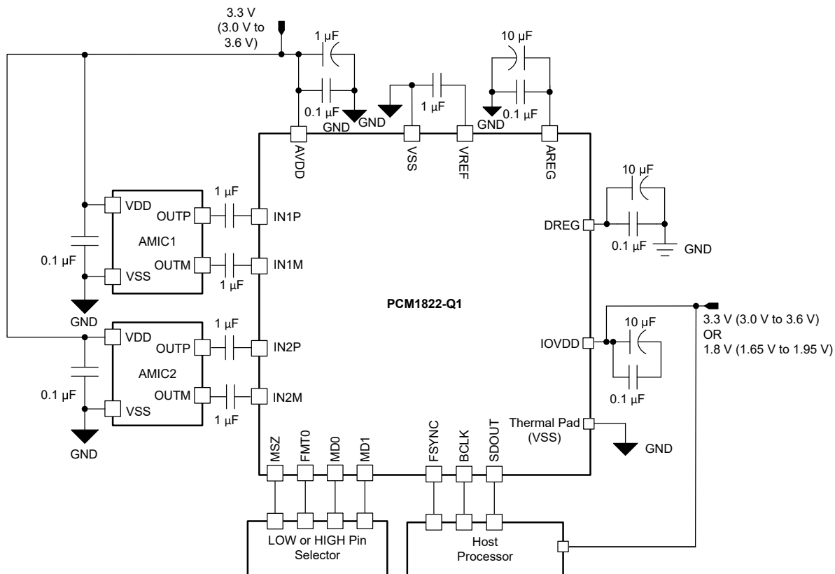
9-1. Two-Channel Analog Microphone Recording Diagram for 3.3-V AVDD Operation
