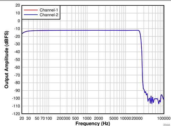
7-6. PCM1820-Q1: Frequency Response With a -12-dBr Input
