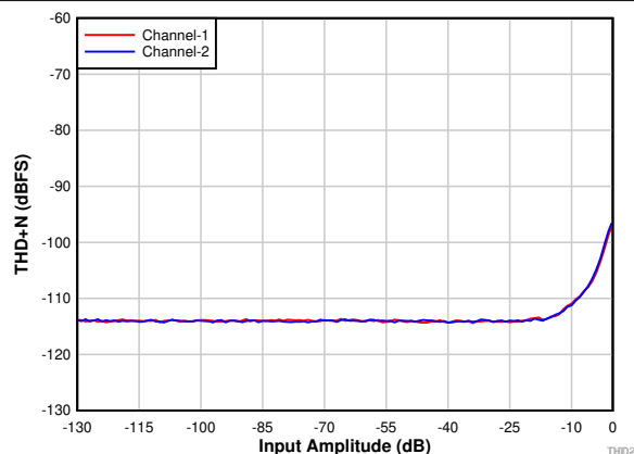
7-2. PCM1820-Q1: THD+N vs Input Amplitude With DRE Disabled
