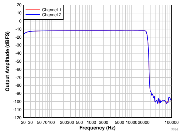
FIG 7-16. PCM1821-Q1: Frequency Response With a -12-dBr Input
