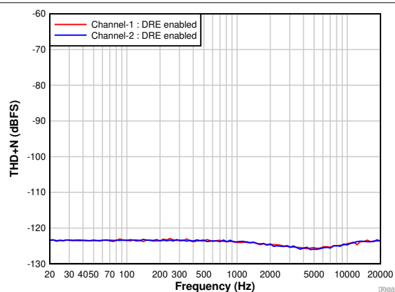
7-3. PCM1820-Q1: THD+N vs Input Frequency With a -60-dBr Input
