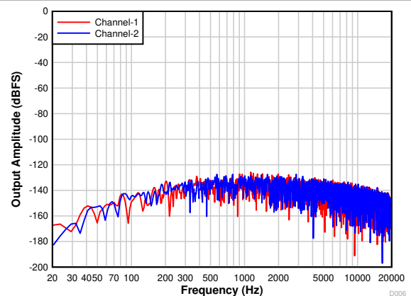
FIG 7-18. PCM1821-Q1: FFT With Idle Input and DRE Disabled
