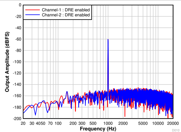
FIG 7-10. PCM1820-Q1: FFT With a -60\text{-dBr} Input and DRE Enabled
