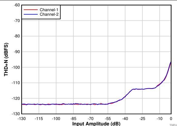
7-1. PCM1820-Q1: THD+N vs Input Amplitude With DRE Enabled
