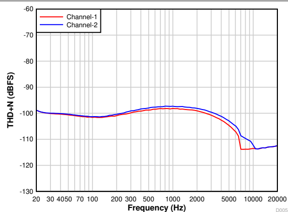
7-5. PCM1820-Q1: THD+N vs Input Frequency With a -1-dBr Input
