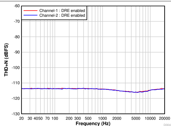
7-4. PCM1820-Q1: THD+N vs Input Frequency With a -60-dBr Input
