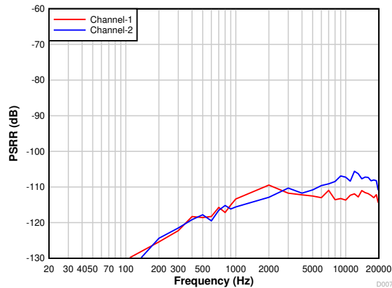
FIG 7-7. PCM1820-Q1: Power-Supply Rejection Ratio vs Ripple Frequency With a 100-mV pp Amplitude
