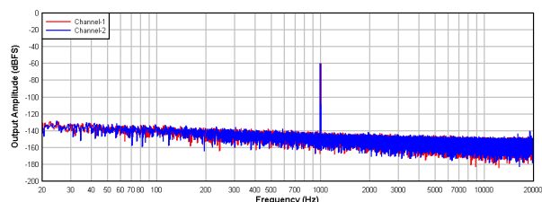
9-6. PCM1821-Q1: FFT With a –60-dBr Input
