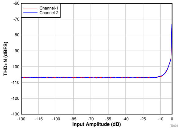
FIG 7-13. PCM1821-Q1: THD+N vs Input Amplitude
