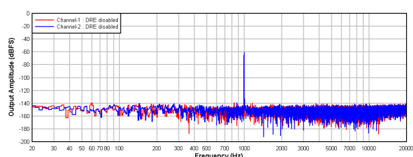
9-4. PCM1820-Q1: FFT With a –60-dBr Input With DRE Disabled
