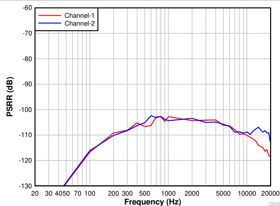
FIG 7-17. PCM1821-Q1: Power-Supply Rejection Ratio With a 100-mV pp Amplitude
