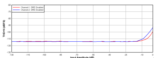
9-5. PCM1820-Q1: THD+N vs Input Amplitude With DRE Disabled
