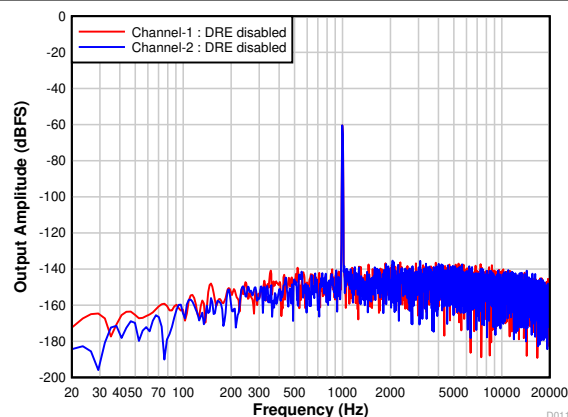
FIG 7-11. PCM1820-Q1: FFT With a -60\text{-dBr} Input and DRE Disabled
