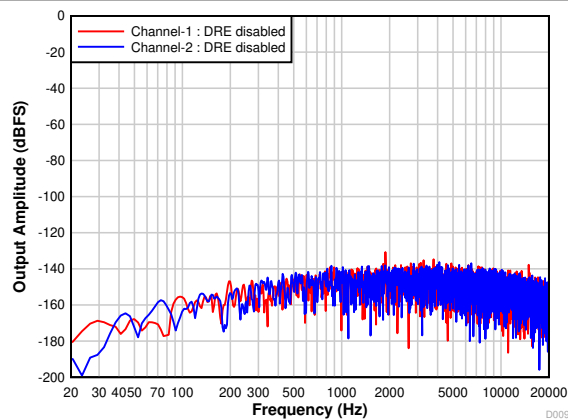
FIG 7-9. PCM1820-Q1: FFT With Idle Input and DRE Disabled
