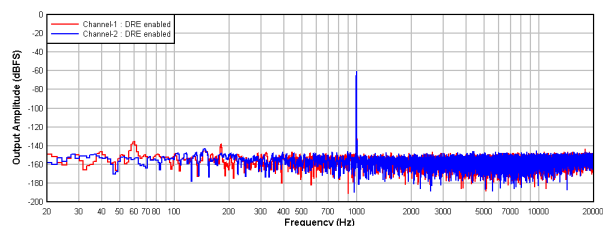
9-2. PCM1820-Q1: FFT With a –60-dBr Input With DRE Enabled
