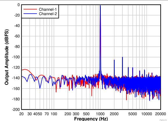
FIG 7-12. PCM1820-Q1: FFT With a -1\text{-dBr} Input
