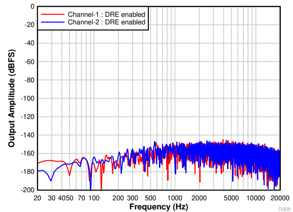
FIG 7-8. PCM1820-Q1: FFT With Idle Input and DRE Enabled
