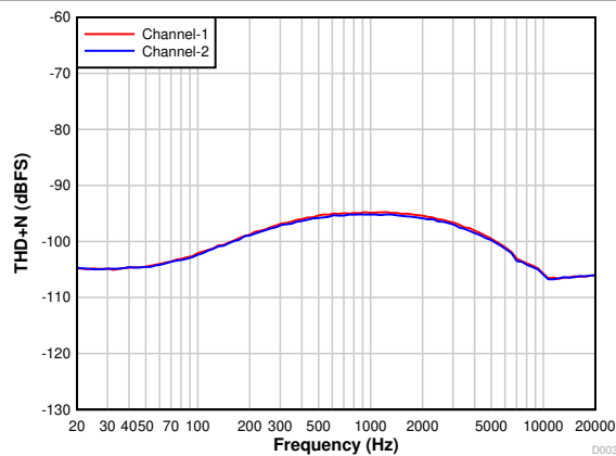
7-15. PCM1821-Q1: THD+N vs Input Frequency With a -1-dBr Input
