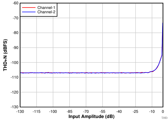
7-13. PCM1821-Q1: THD+N vs Input Amplitude
