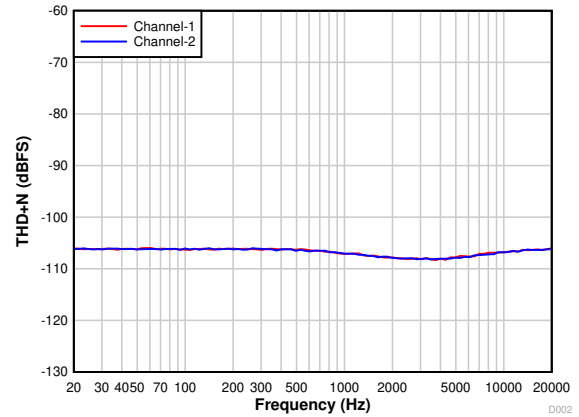
7-14. PCM1821-Q1: THD+N vs Input Frequency With a -60-dBr Input
