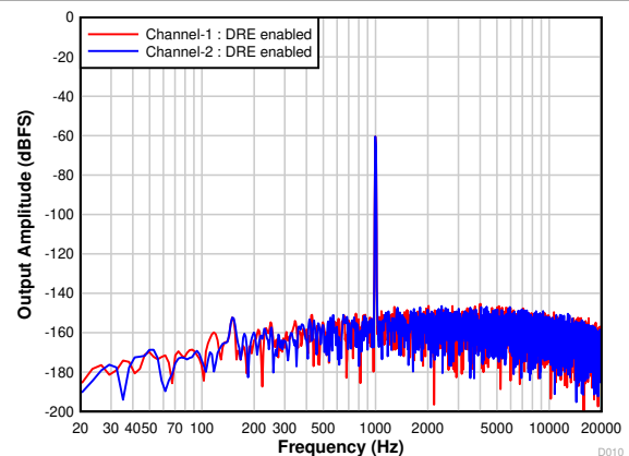
FIG 7-10. PCM1820-Q1: FFT With a -60-dBr Input and DRE Enabled
