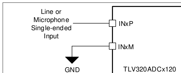
図 6-7. Single-Ended, DC-Coupled Input Connection
