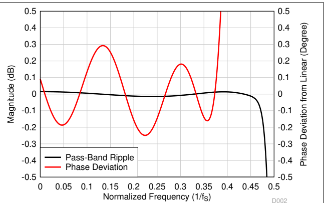
図 6-32. Low-Latency Decimation Filter Pass-Band Ripple and Phase Deviation
