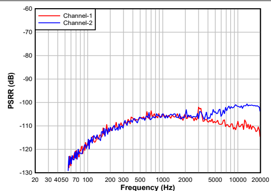
5-6. Single-ended Input: PSRR vs. frequency with AC Coupled input
