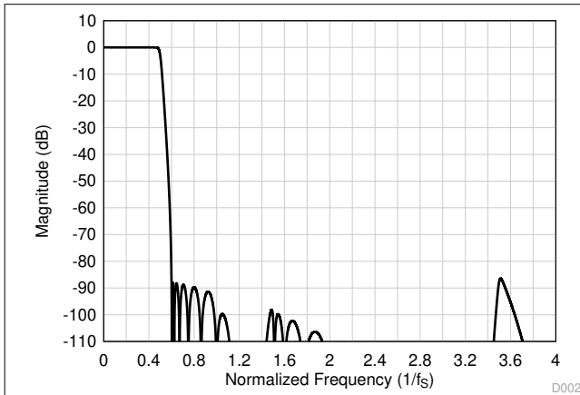
図 6-31. Low-Latency Decimation Filter Magnitude Response
