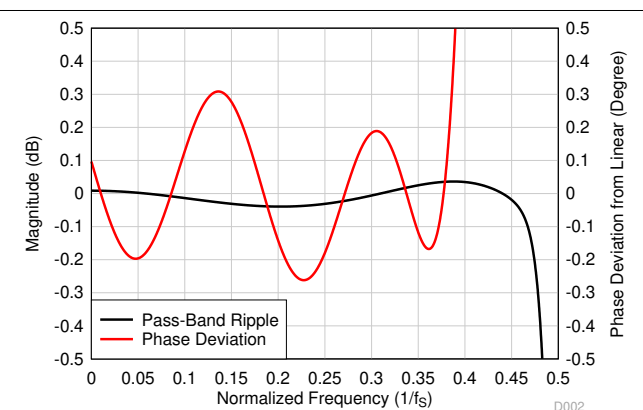
図 6-30. Low-Latency Decimation Filter Pass-Band Ripple and Phase Deviation
