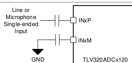
図 6-8. Single-Ended, AC-Coupled Input Connection
