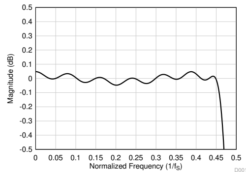
図 6-16. Linear Phase Decimation Filter Pass-Band Ripple
