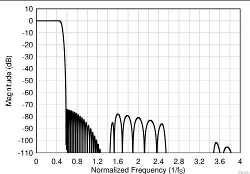
図 6-17. Linear Phase Decimation Filter Magnitude Response
