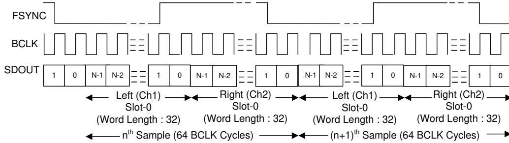
図 6-6. I 2 S Protocol Timing In Controller Mode
