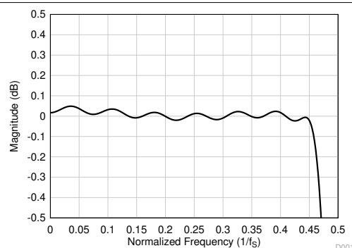
図 6-12. Linear Phase Decimation Filter Pass-Band Ripple
