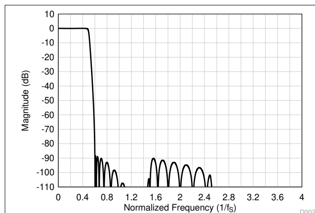
図 6-29. Low-Latency Decimation Filter Magnitude Response
