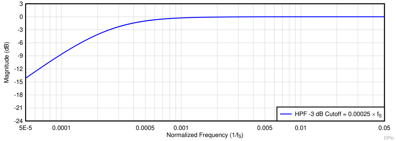
6-10. HPF Filter Frequency Response Plot
