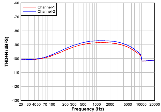
5-2. Single-ended Input: THD+N vs Frequency With DC Coupled -1dBFS signal
