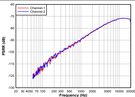
5-5. Single-ended Input: PSRR vs. Frequency with DC Coupled input
