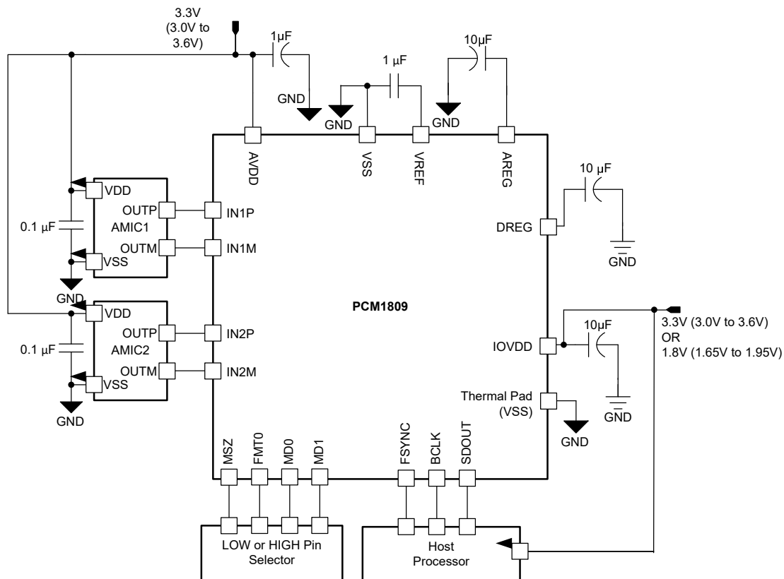
図 7-1. Two-Channel Analog Microphone Recording Diagram for 3.3-V AVDD Operation
