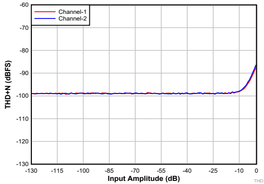
5-1. Single-ended Input: THD+N vs Input Amplitude With DC Coupled signal(non A-weighted)
