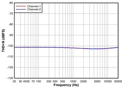
5-3. Single-ended Input: DR vs Input Frequency With DC Coupled signal
