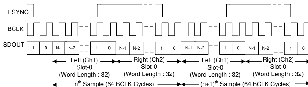
図 6-6. I 2 S Protocol Timing In Controller Mode
