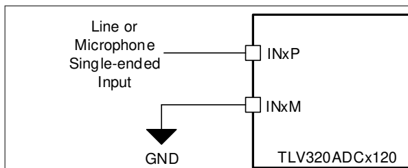
図 6-7. Single-Ended, DC-Coupled Input Connection
