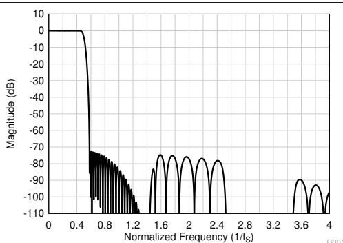
図 6-11. Linear Phase Decimation Filter Magnitude Response
