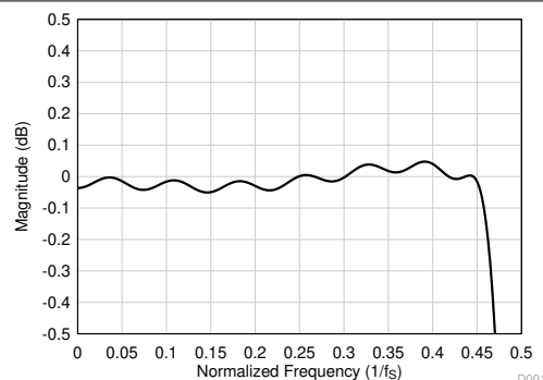
図 6-18. Linear Phase Decimation Filter Pass-Band Ripple
