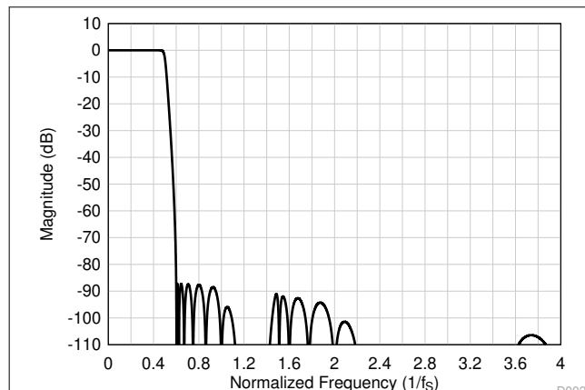
図 6-27. Low-Latency Decimation Filter Magnitude Response
