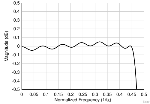
図 6-14. Linear Phase Decimation Filter Pass-Band Ripple
