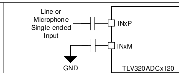
図 6-8. Single-Ended, AC-Coupled Input Connection
