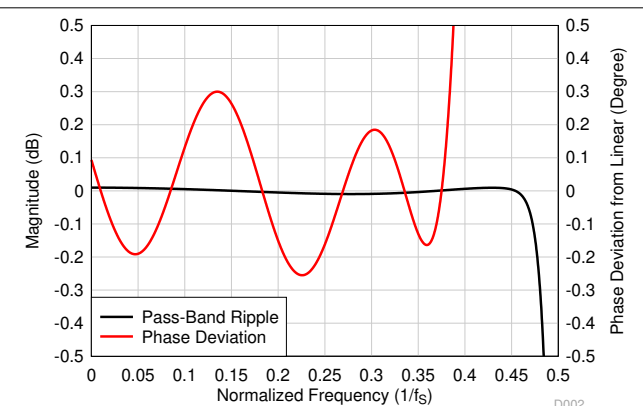
図 6-28. Low-Latency Decimation Filter Pass-Band Ripple and Phase Deviation
