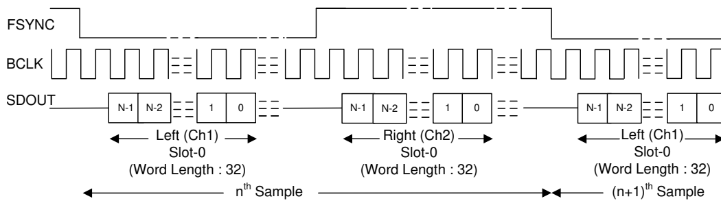
図 6-5. I 2 S Mode Protocol Timing in Target Mode
