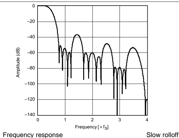
Figure 4. Amplitude vs Frequency
