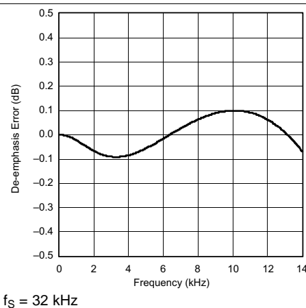
Figure 7. De-Emphasis Error vs Frequency
