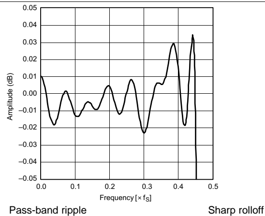
Figure 3. Amplitude vs Frequency
