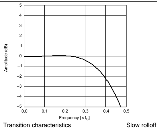
Figure 5. Amplitude vs Frequency
