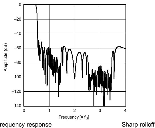
Figure 2. Amplitude vs Frequency
