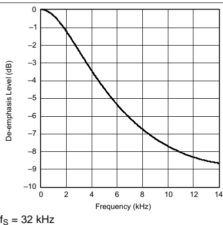
Figure 6. De-Emphasis Level vs Frequency
