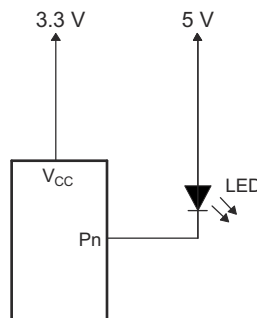
図 9-3. Device Supplied By Lower Voltage
