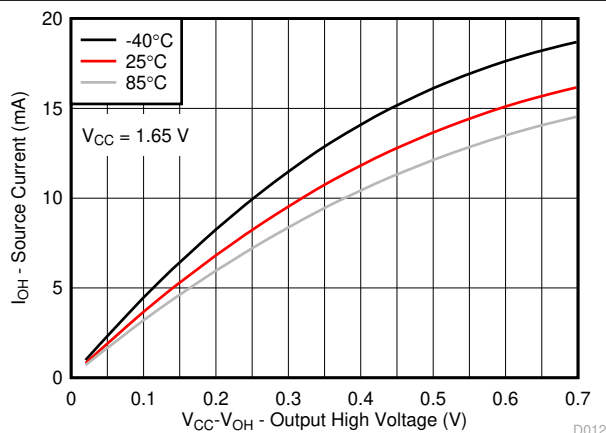
FIG 6-11. I/O Source Current vs Output High Voltage for Different Temperature ( T_A ) for V_{CC} = 1.65\text{ V}
