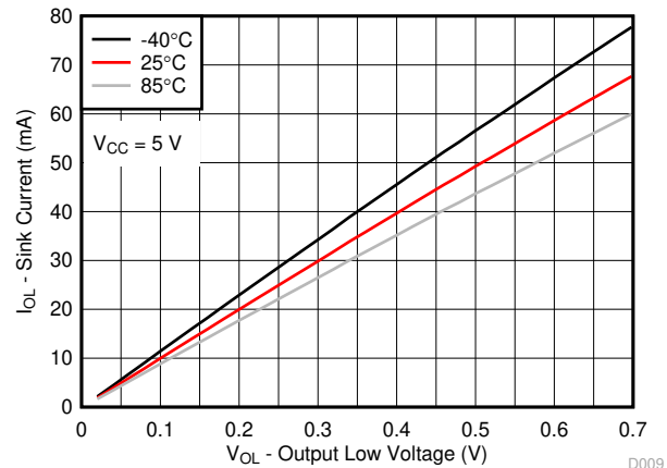
FIG 6-8. I/O Sink Current vs Output Low Voltage for Different Temperature ( T_A ) for V_{CC} = 5\text{ V}
