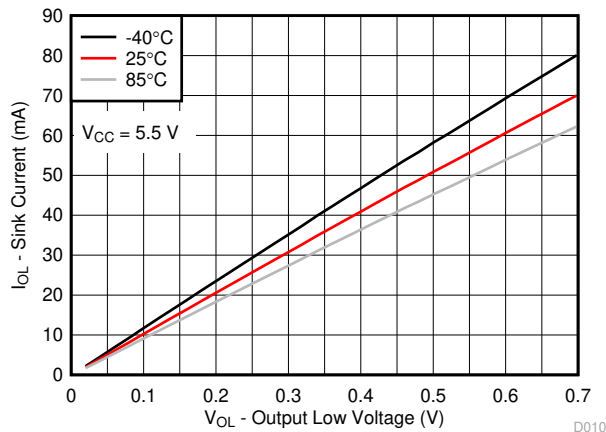
FIG 6-9. I/O Sink Current vs Output Low Voltage for Different Temperature ( T_A ) for V_{CC} = 5.5\text{ V}
