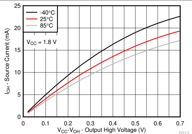
FIG 6-12. I/O Source Current vs Output High Voltage for Different Temperature ( T_A ) for V_{CC} = 1.8\text{ V}
