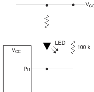
図 9-2. High-Value Resistor In Parallel With Led
