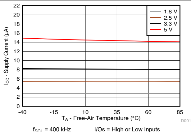
6-1. Supply Current ( I_{\text{CC}} , Operating Mode) vs Temperature ( T_A ) at Four Supply Voltages
