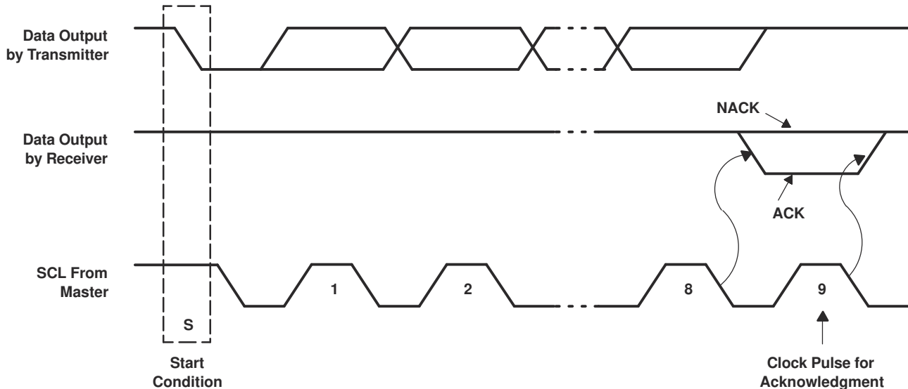
图 8-5. Acknowledgment On The I²C Bus
