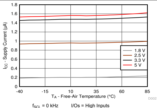
6-2. Supply Current ( I_{\text{CC}} , Standby Mode) vs Temperature ( T_A ) at Four Supply Voltages
