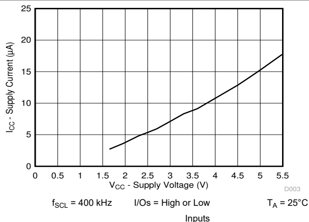
6-3. Supply Current ( I_{\text{CC}} , Operating Mode) vs Supply Voltage ( V_{\text{CC}} )
