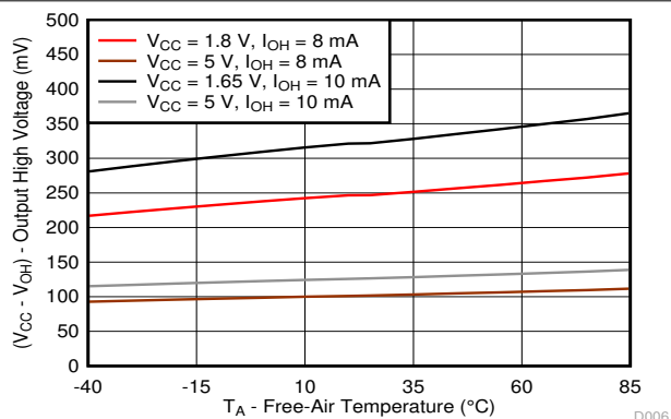
6-6. Output High Voltage ( V_{\text{CC}} - V_{\text{OH}} ) vs Temperature ( T_A ) for P-Ports
