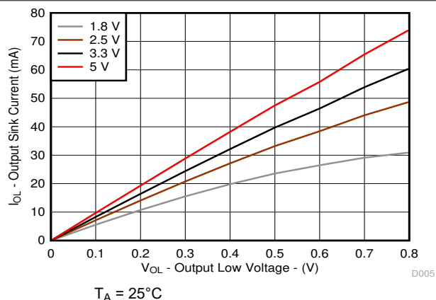
6-5. Sink Current ( I_{\text{OL}} ) vs Output Low Voltage ( V_{\text{OL}} ) for P-Ports at Four Supply Voltages
